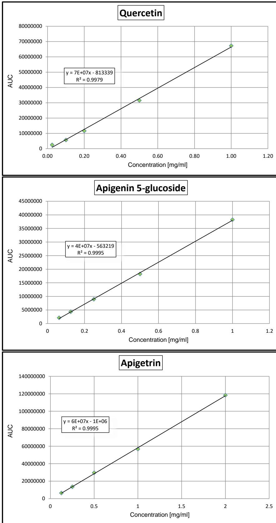
Figure S1. The calibration curves of detected compounds.
