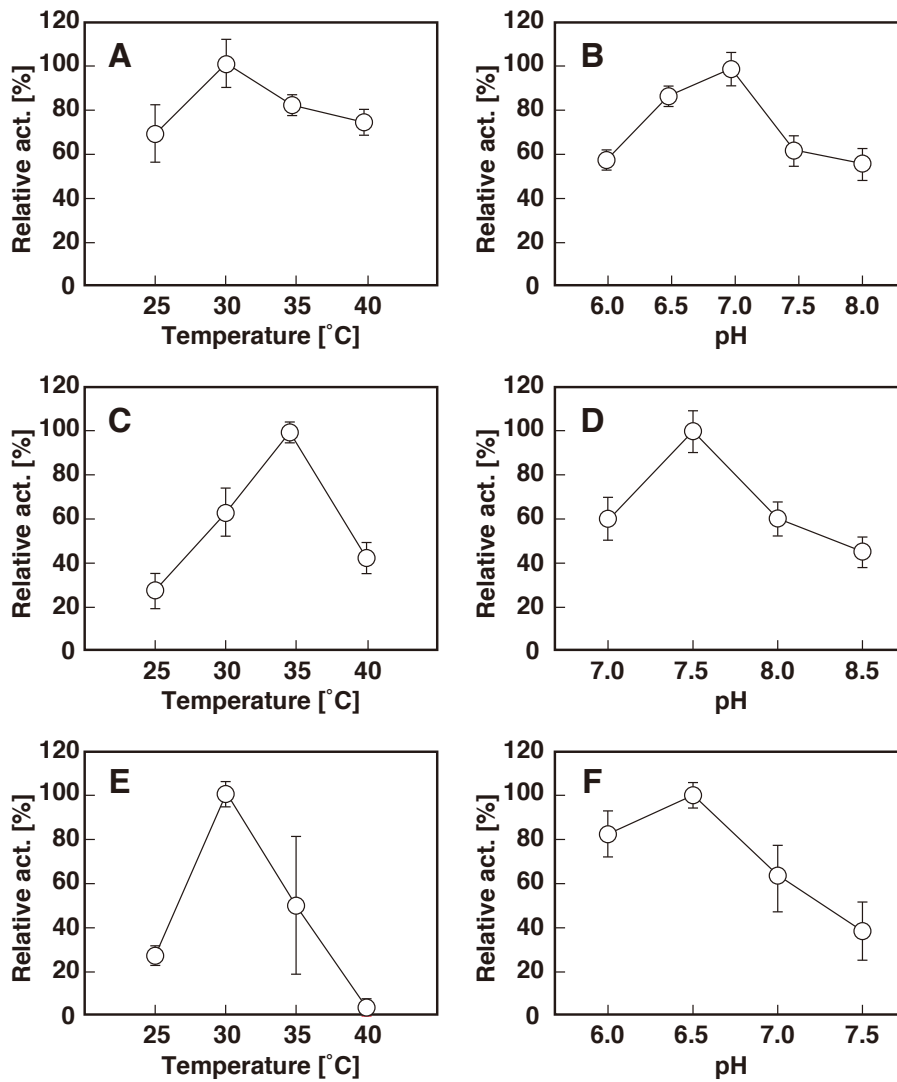
Fig. S1. Effect of temperature (A, C, and E) and pH (B, D, and F) on Lcp activity. Relative oxygen consumption activities of Lcp1-his (A and B), Lcp2-his (C and D), and Lcp3-his (E and F) were indicated. Each value is the average \pm standard deviation of three independent experiments performed in parallel.
