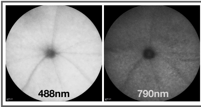
Dual vector 2E+10
