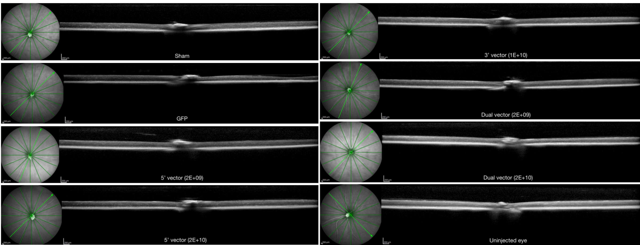
Supplementary Figure 5. Example OCT scans of injected eyes taken 6 months post-injection through the region of injection for each cohort.
