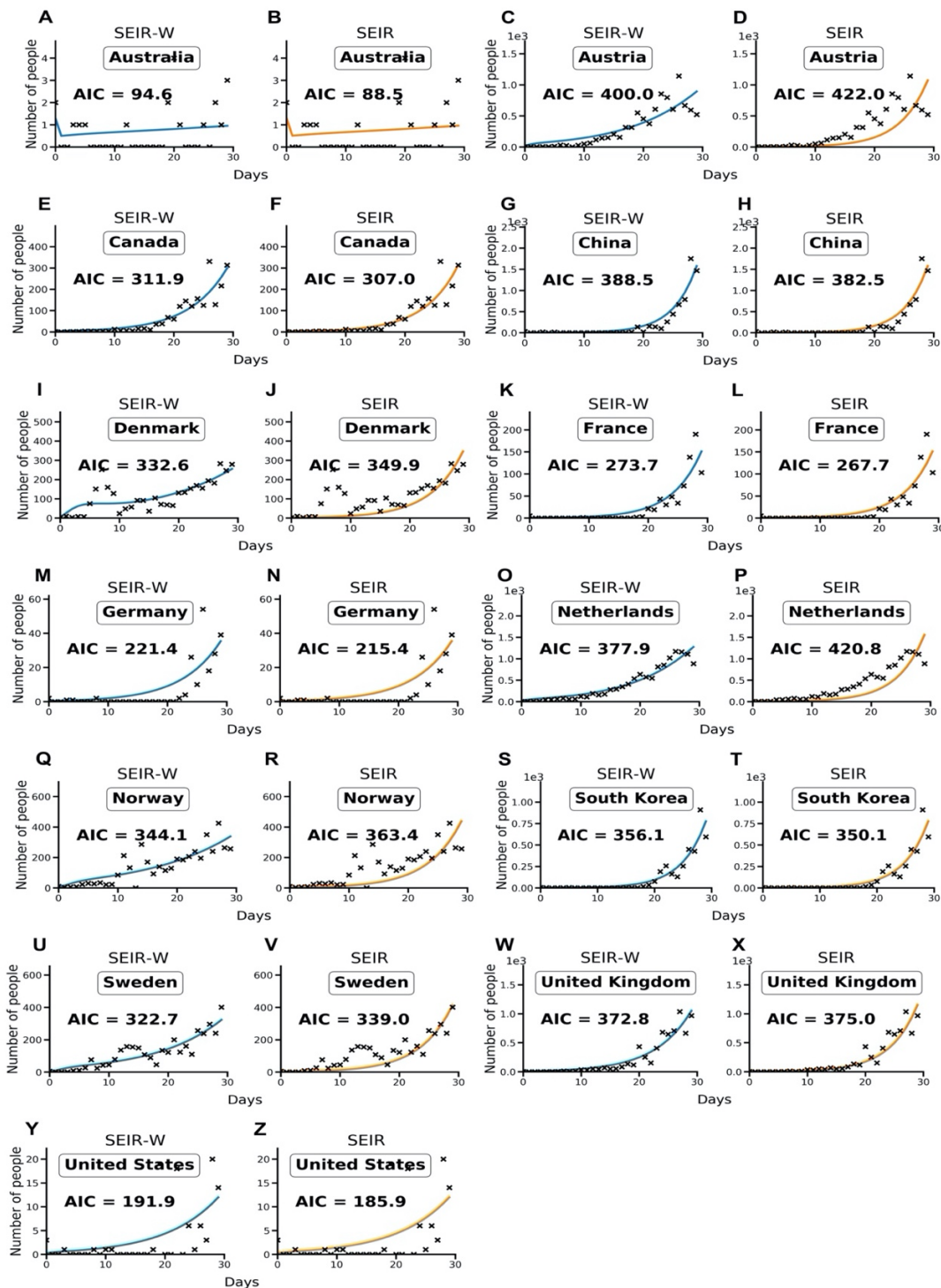
Fig. S2. Graphical depiction of data in the Table S4. A-Z correspond to 13 country fits of the mathematical models—SEIR and SEIR-W. Four other country fits are depicted in the main text Fig. 1 (Spain, Italy, Iran, Switzerland).
