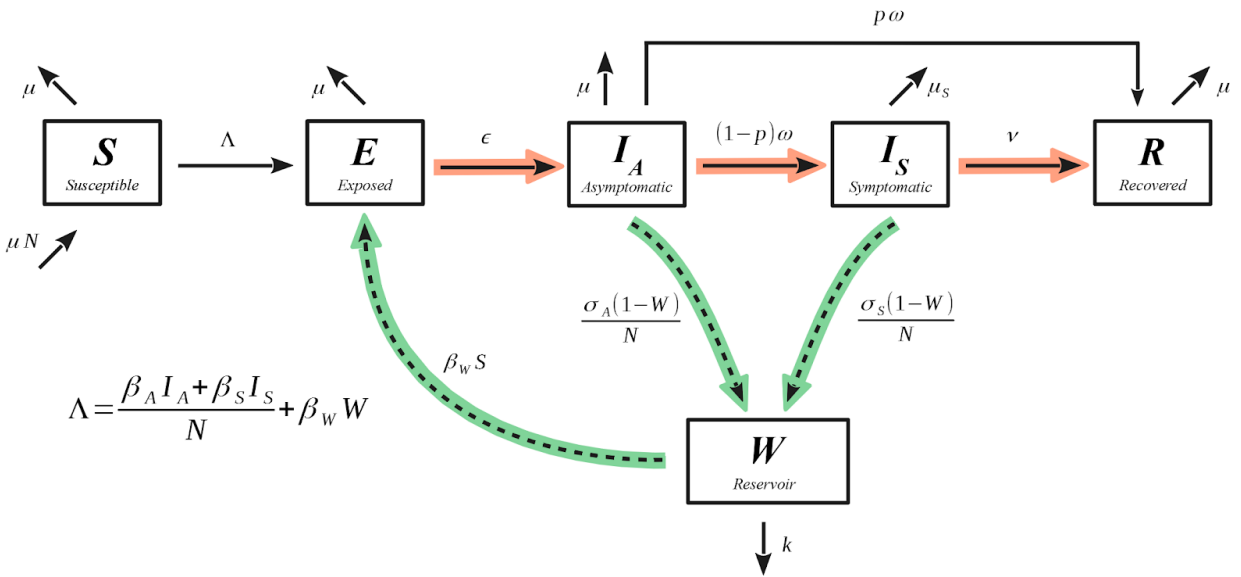
Fig. S1. SEIR-W model for SARS-CoV-2 transmission. Compartmental diagram with dynamic information, where the green highlighted arrows represent how the infection couples with the environment, and the red highlighted arrows represent the progression of the infection through individuals. The model is referred to as SEIR-W throughout the text.
