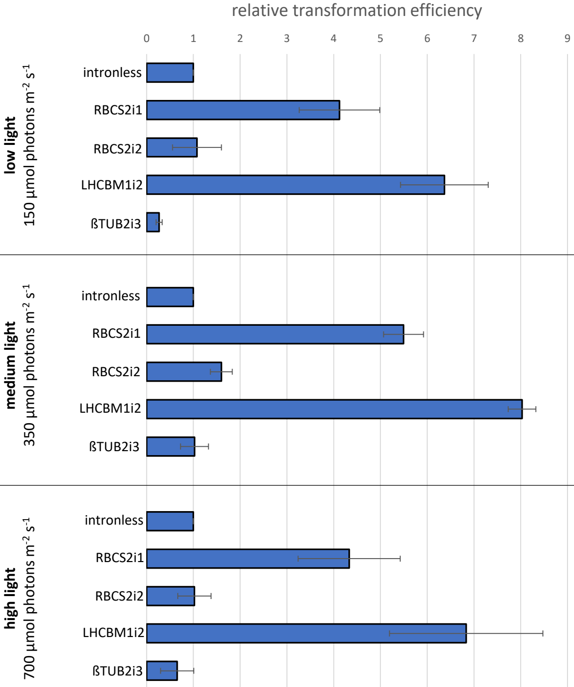
S2 Fig: Relative transformation efficiency of four selected introns (RBCS2i1 RBCS2i2, LHCBM1i2 and \beta TUB2i3) with different IME capacities. Selection after transformation was performed at different light intensities (150, 350 and 700 \mu\text{mol photons m}^{-2} \text{s}^{-1} ). Data represents the mean of biological triplicates.
