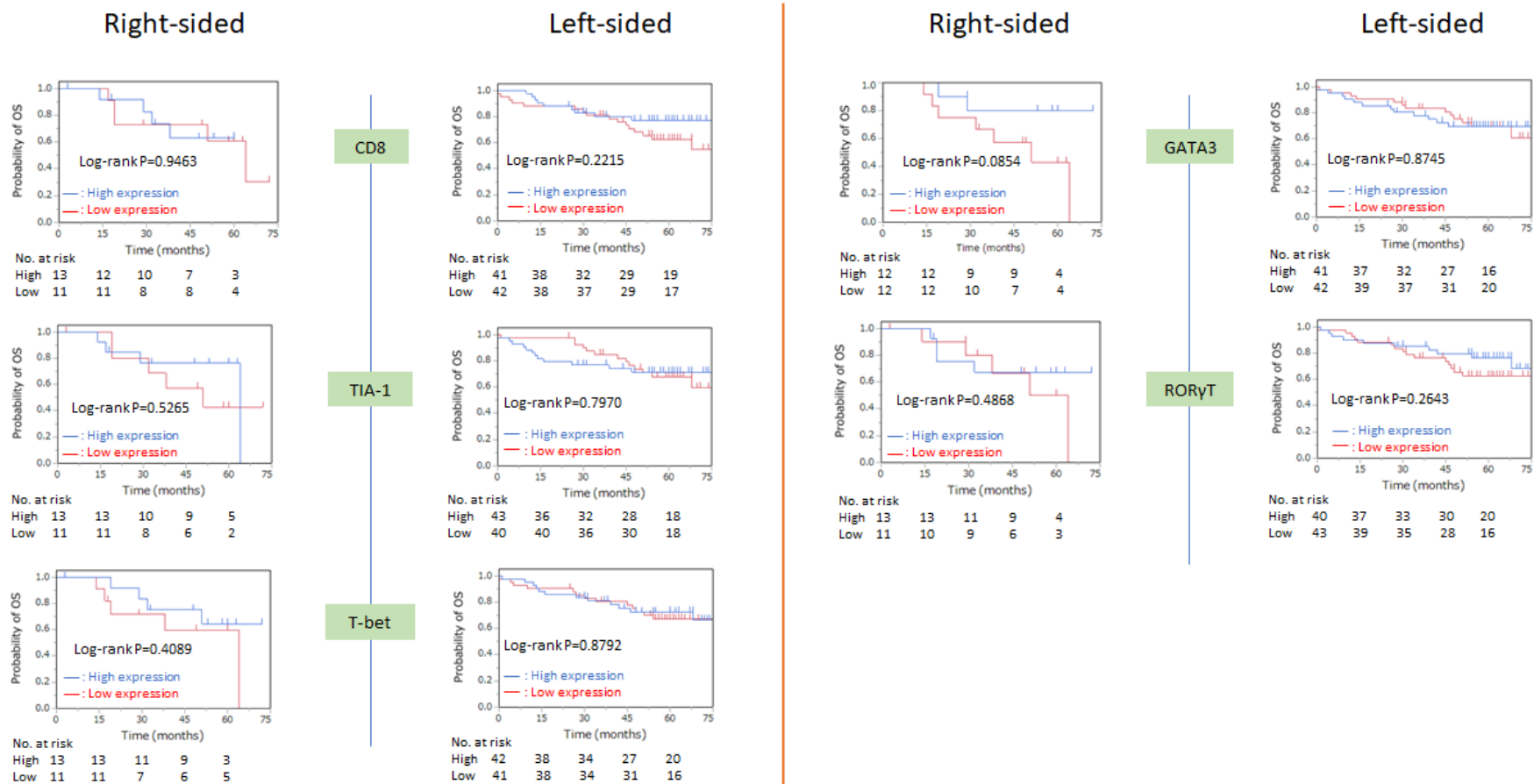
Figure S9. Kaplan-Meier curves of overall survival (OS) according to tumor sidedness, excluding MMR deficiency, based on the molecular expression of CD8, TIA-1, T-bet, GATA3, and RORγT. The median values were used as the cut-off point.
