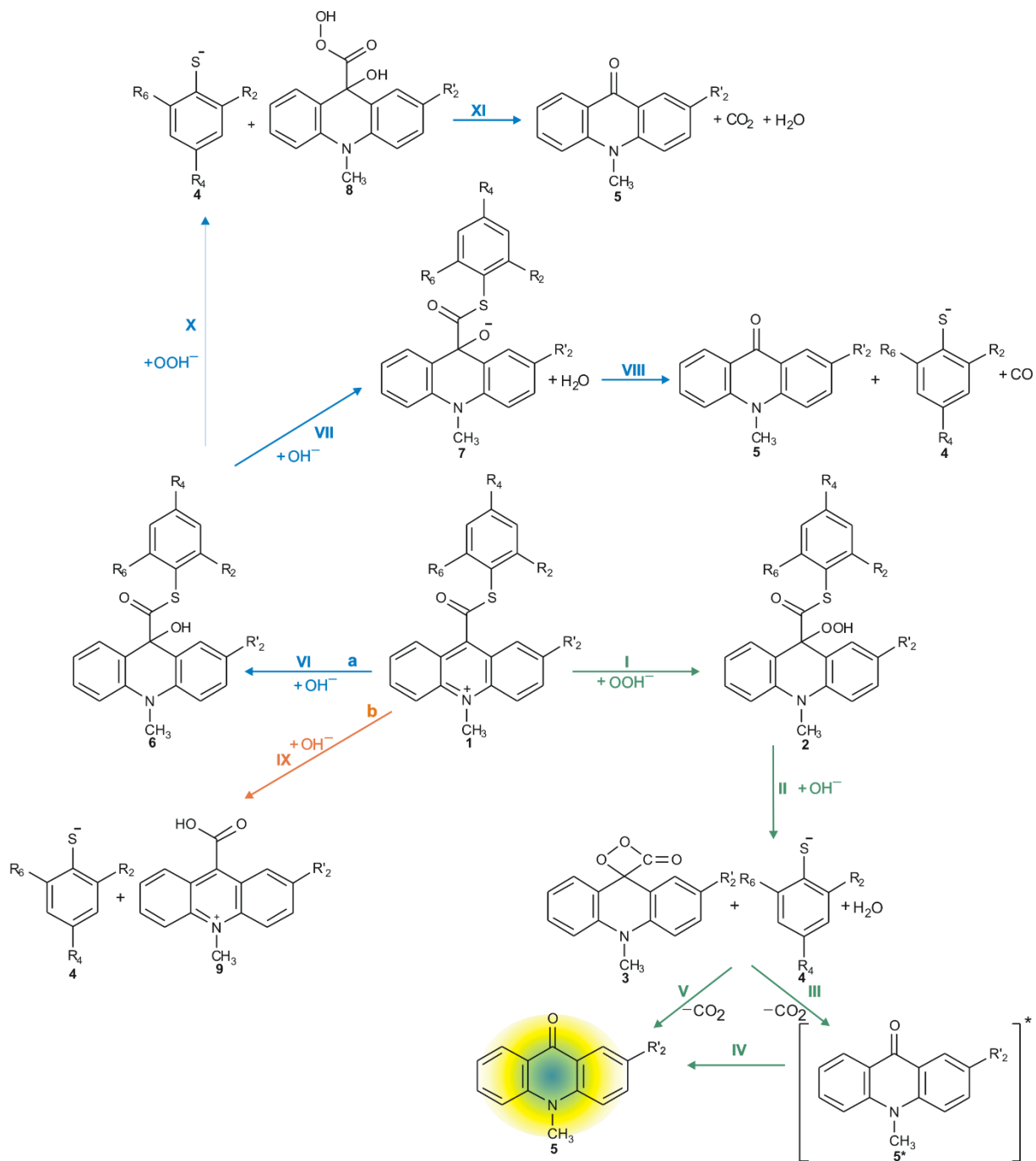
Scheme S1. Pathways of the reactions of ATE with \text{OOH}^- and \text{OH}^- (CL pathway (green arrows), non-CL pathways: transformation of ATE to the non-emitting product (blue arrows) and hydrolysis of ATE (orange arrows)).
