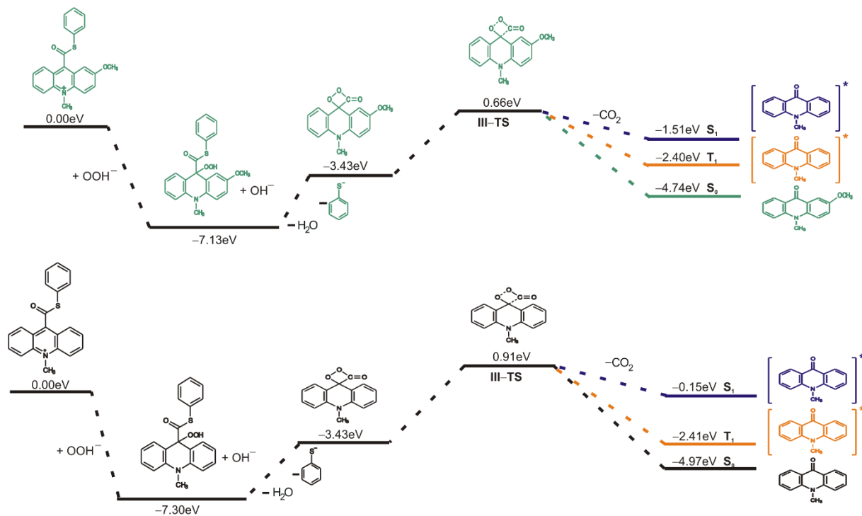
Figure S3. Energy diagram of the chemiluminescence reaction in the gaseous phase with energy of the lowest triplet ( T_1 ) and singlet ( S_1 ) states.
