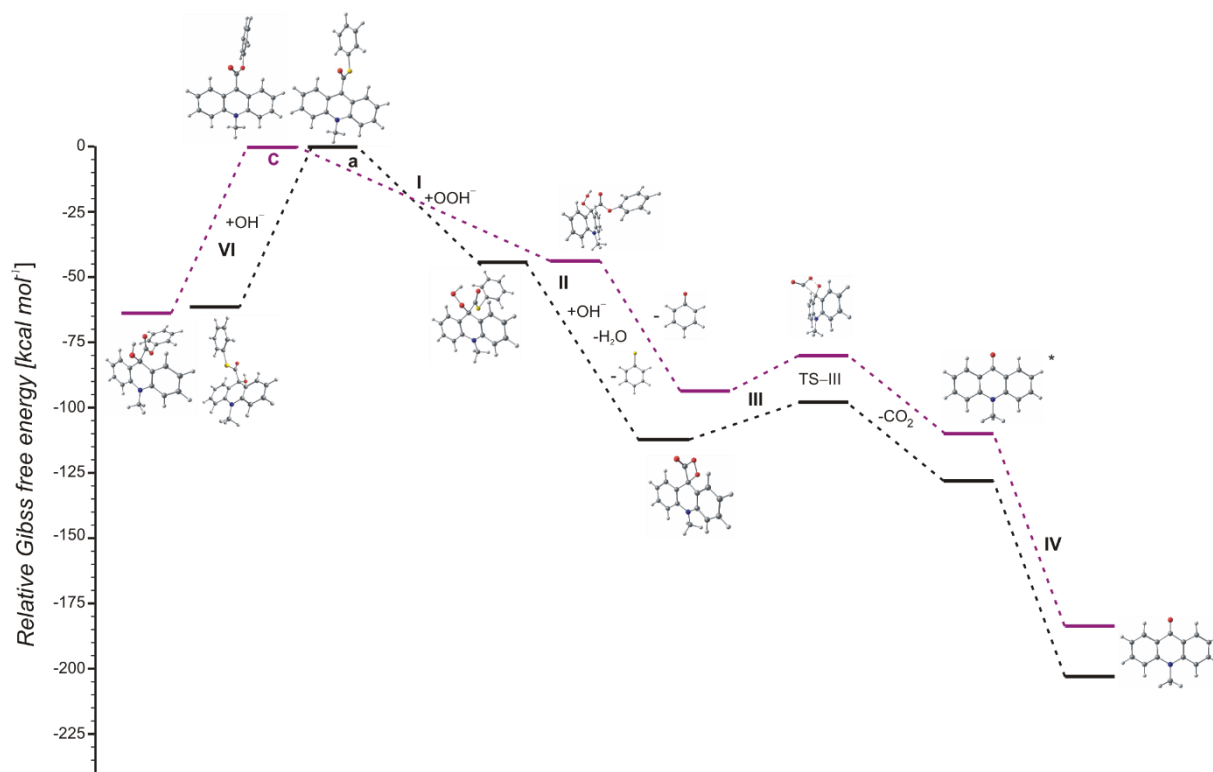
Figure S2. Relative Gibbs free energies of the CL pathway (reaction steps: I–IV) and non-CL step VI (formation of pseudobase) of acridinium thioesters: (a, black) and acridinium esters (c, violet).
