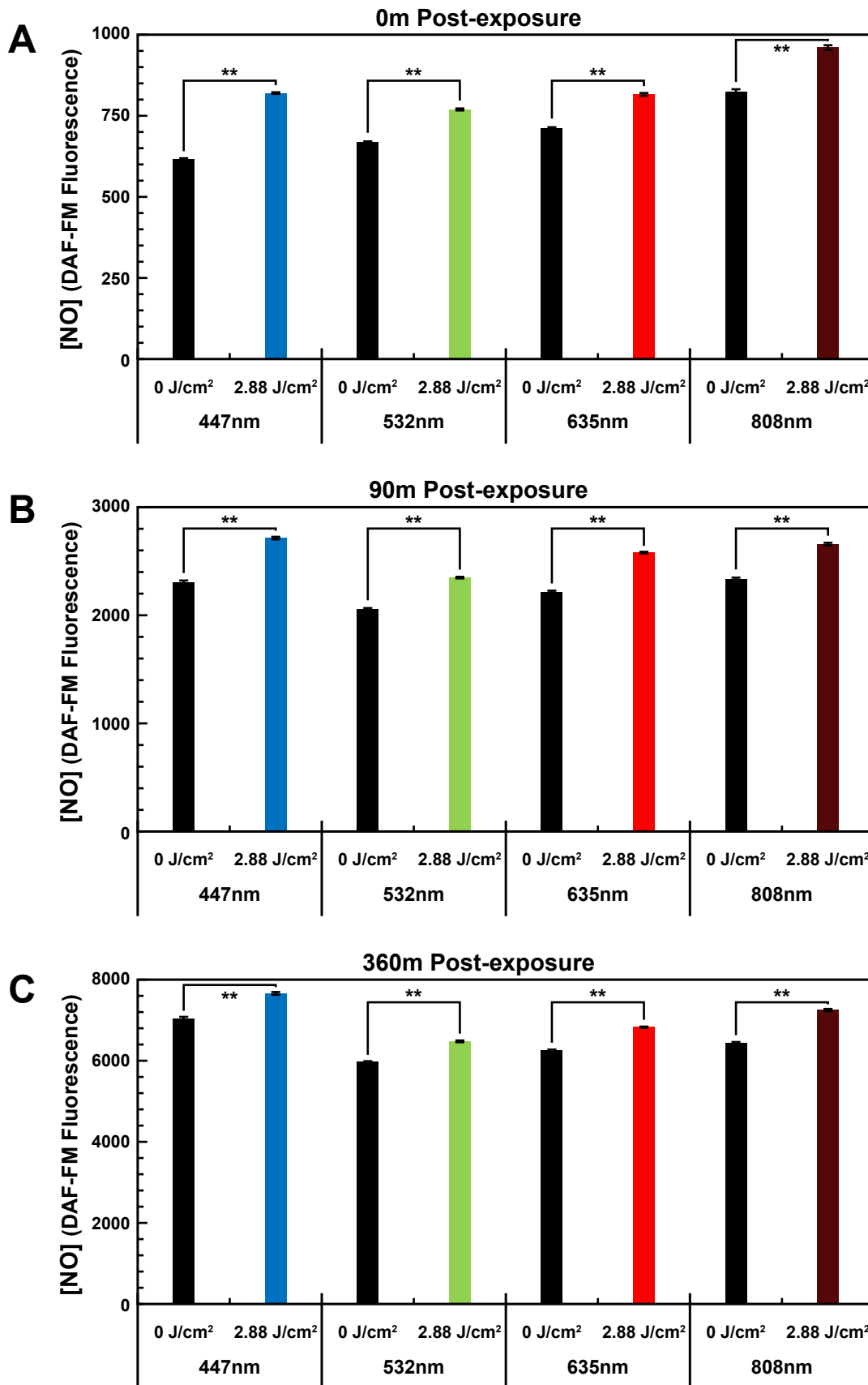
Fig S1. Raw DAF-FM fluorescence values following light exposure. (A) Graph of DAF-FM fluorescence \pm standard error immediately following exposure to 2.88 \pm 0.06 J/cm 2 of 447 nm (n=44), 532 nm (n=52), 635 nm (n=48), or 808 nm (n=56) light (all at an irradiance of 800 \pm 17.9 \mu W/cm 2 ) and corresponding unexposed controls. (B) DAF-FM fluorescence remains elevated at 90 min and (C) 360 min post-exposure. ** p<0.001.
