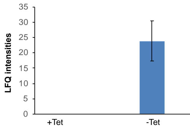
Figure S3. Silencing of TrypOx transcript resulted in no protein synthesis. TrypOx protein intensities TrypOx/RNAi strains in absence (uninduced) and presence (induced) tetracycline. Protein identification and intensities were measured using LC-MS/MS in three biological replicates.
