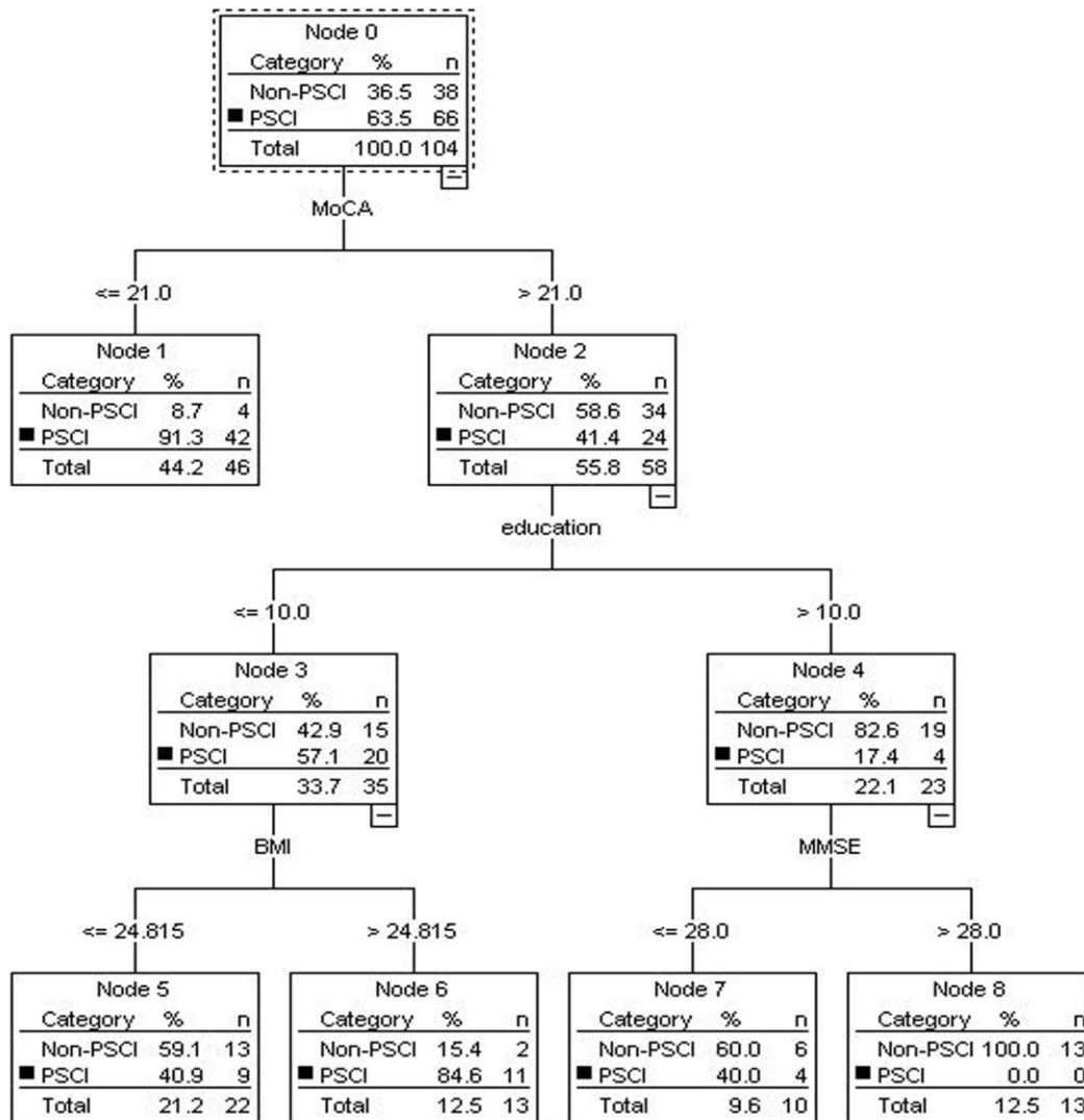
Figure S1. A decision tree model for the prediction of cognitive impairment at 3 to 6 months after the onset of stroke that includes baseline MoCA scores, educational level, body mass index (BMI), and baseline MMSE scores.
