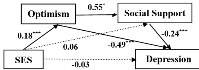
FIGURE S1 Another Serial-mediation model with optimism as an antecedent of social support. Standardized coefficients were presented. The dotted lines denote insignificant direct effect from SES to depression and insignificant indirect effect of social support in the SES-depression linkage. * p < 0.05 , *** p < 0.001 .
