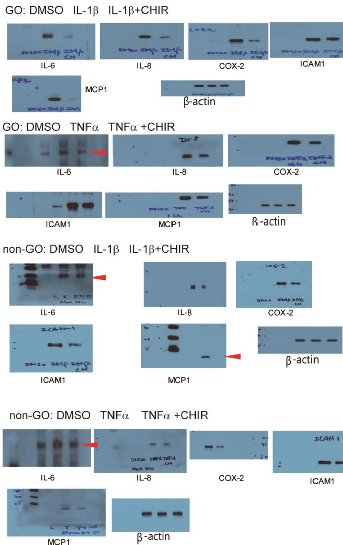
Supplementary figure 3. Full-length western blot of Figure 5. The red arrowheads are drawn to indicate the bands for IL-6 and MCP-1. The first section captioned ‘GO: DMSO, IL-1 \beta , IL-1 \beta +CHIR’ corresponds to the first column of blot images of Figure 5A. The bands within each full length image are in the order of treatment with DMSO, IL-1 \beta and IL-1 \beta with CHIR. The second section captioned ‘GO: DMSO TNF- \alpha TNF- \alpha +CHIR’ are full length immunoblots of the second column of Figure 5A. The third section captioned ‘non-GO: DMSO IL-1 \beta IL-1 \beta +CHIR’ corresponds to the third column, and the fourth section captioned ‘non-GO DMSO TNF- \alpha TNF- \alpha +CHIR’ corresponds to the fourth column.
