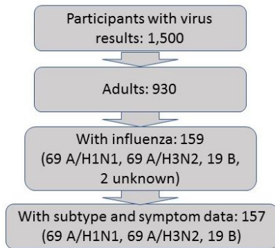
Supplemental Figure 1. Flow chart of data inclusion for analysis of symptom data collected in ARIC study.
