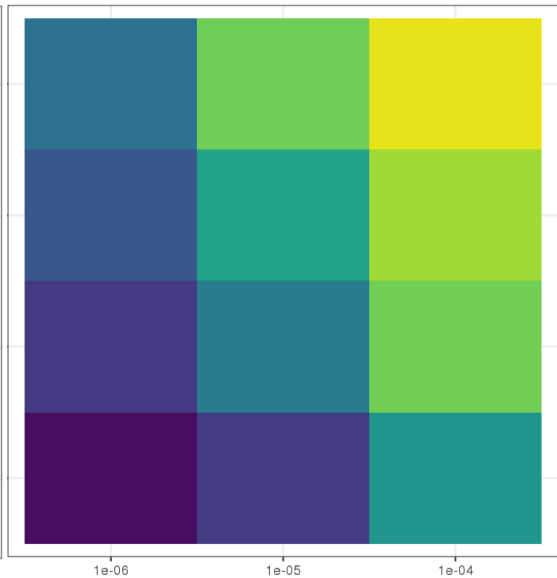
Deme size = 4096
