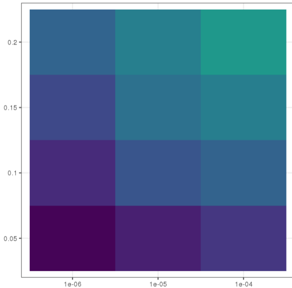
Deme size = 64
