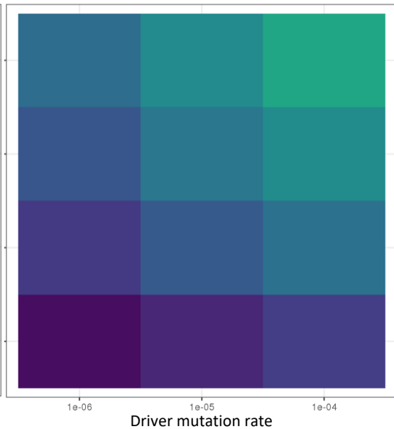
Deme size = 512
