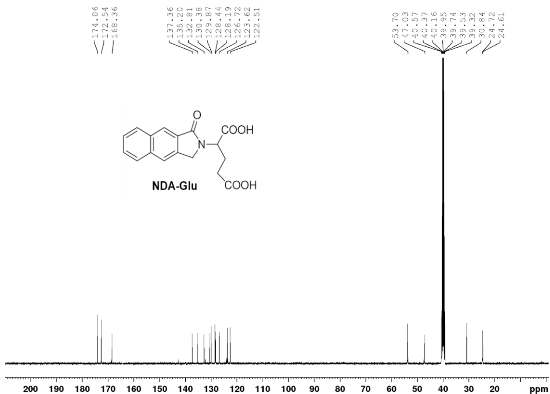
Fig. S17 13 C NMR spectrum of NDA-Glu.
