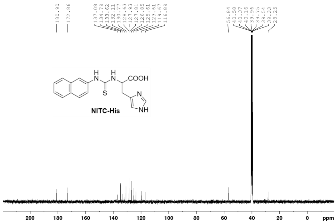
Fig. S37 13 C NMR spectrum of NITC-His.
