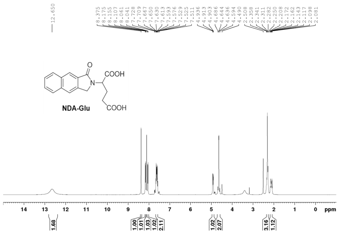
Fig. S16 1 H NMR spectrum of NDA-Glu.
