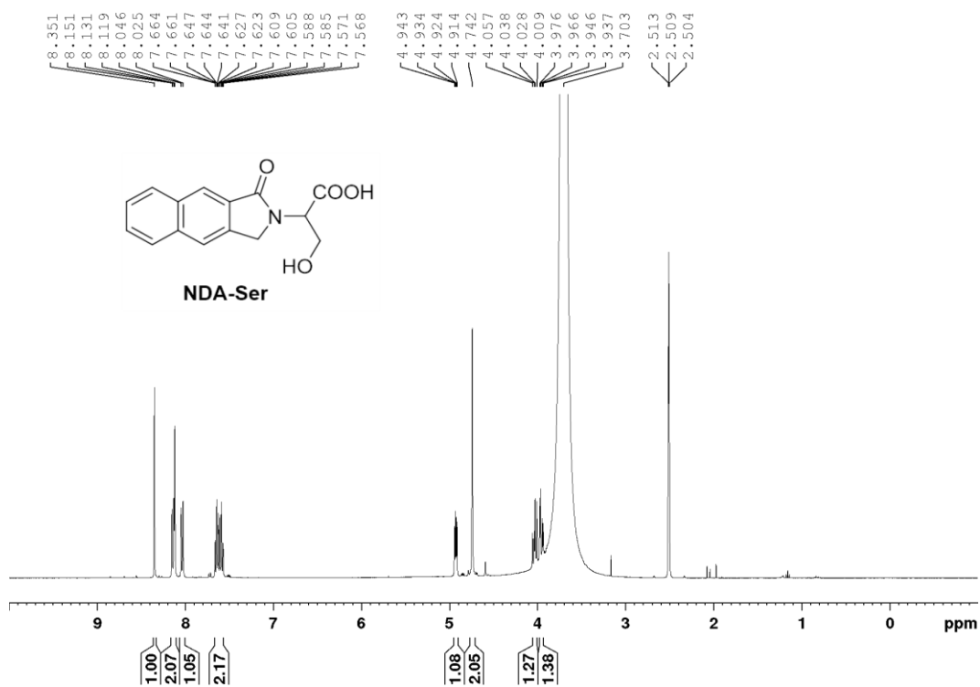
Fig. S10 1 H NMR spectrum of NDA-Ser.
