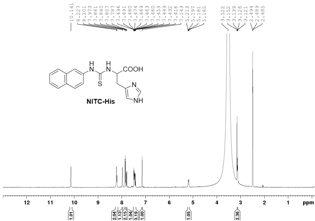
Fig. S36 1 H NMR spectrum of NITC-His.
