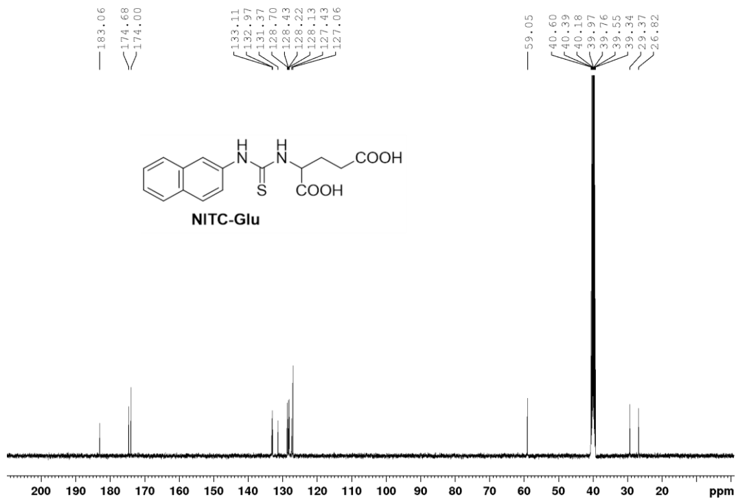
Fig. S35 ^{13}\text{C} NMR spectrum of NITC-Glu.
