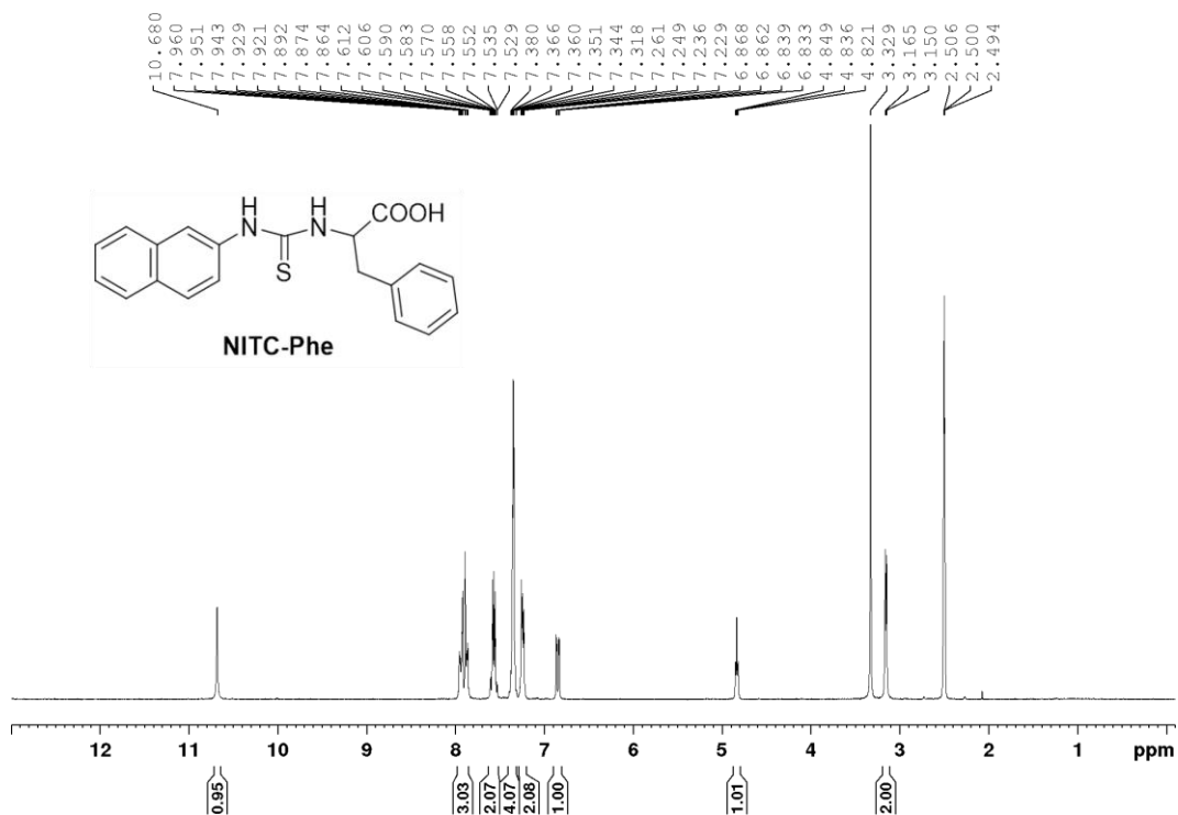
Fig. S30 ^1\text{H} NMR spectrum of NITC-Phe.
