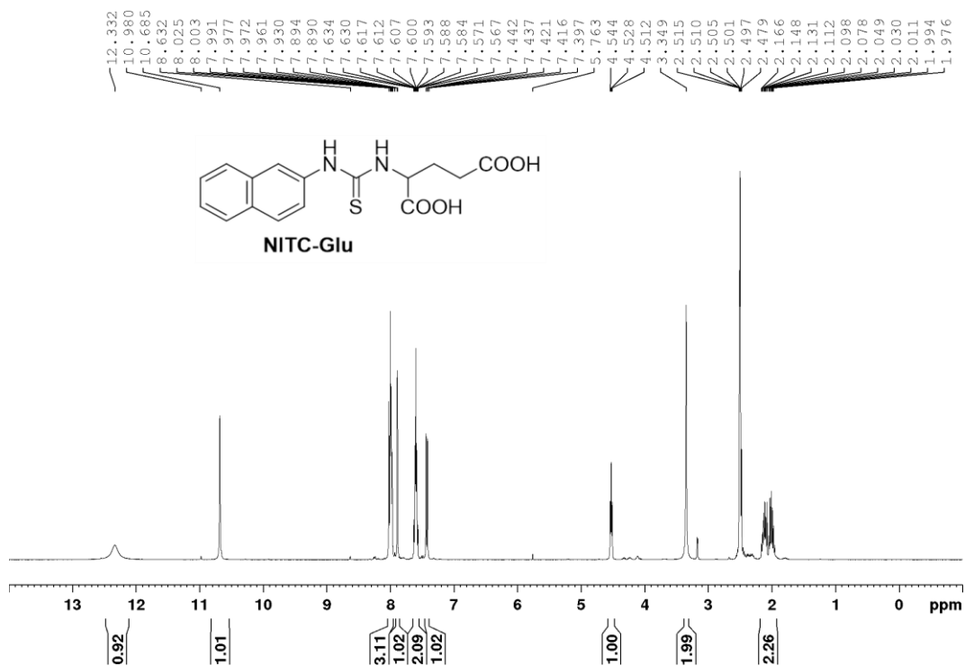
Fig. S34 ^1\text{H} NMR spectrum of NITC-Glu.
