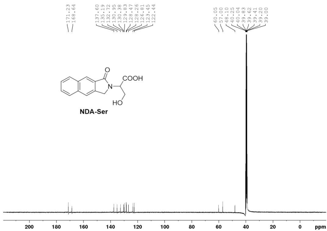
Fig. S11 13 C NMR spectrum of NDA-Ser.
