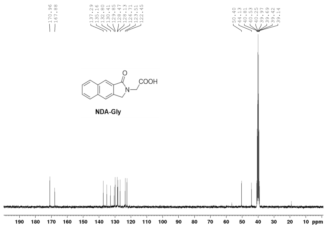
Fig. S5 13 C NMR spectrum of NDA-Gly.
