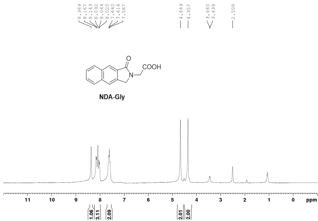
Fig. S4 1 H NMR spectrum of NDA-Gly.
