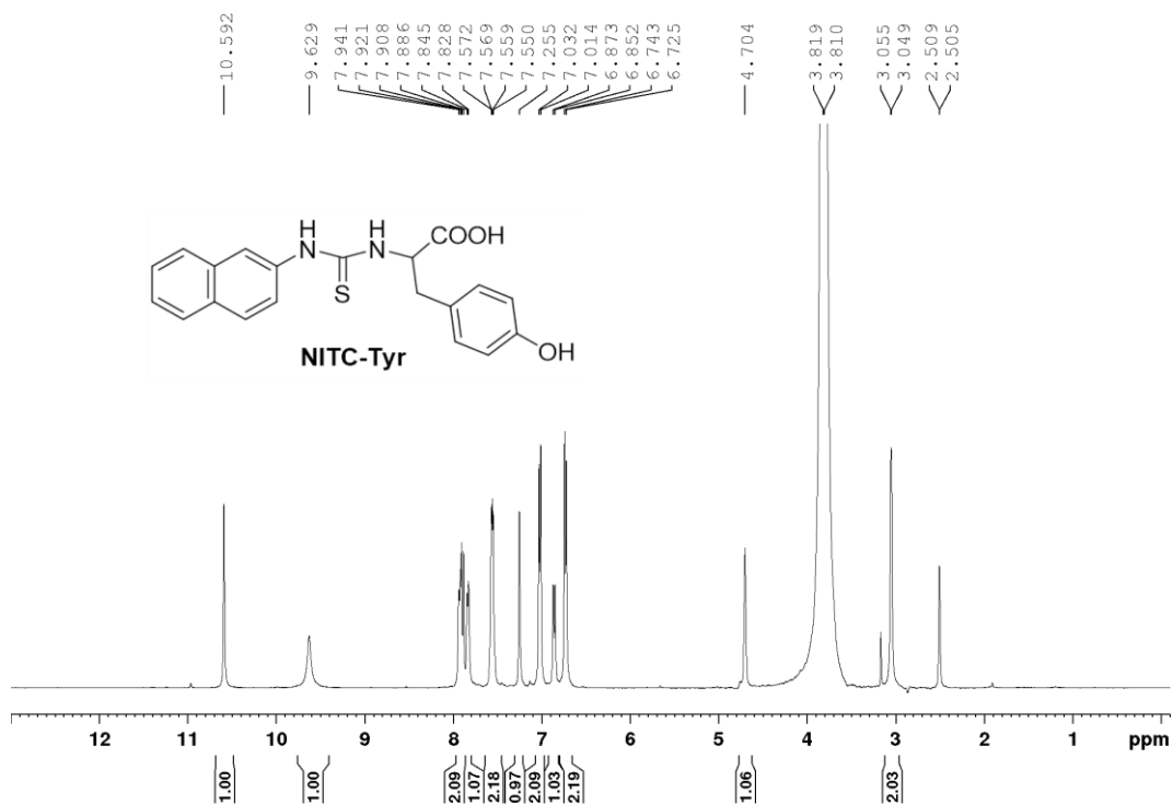
Fig. S32 1 H NMR spectrum of NITC-Tyr.
