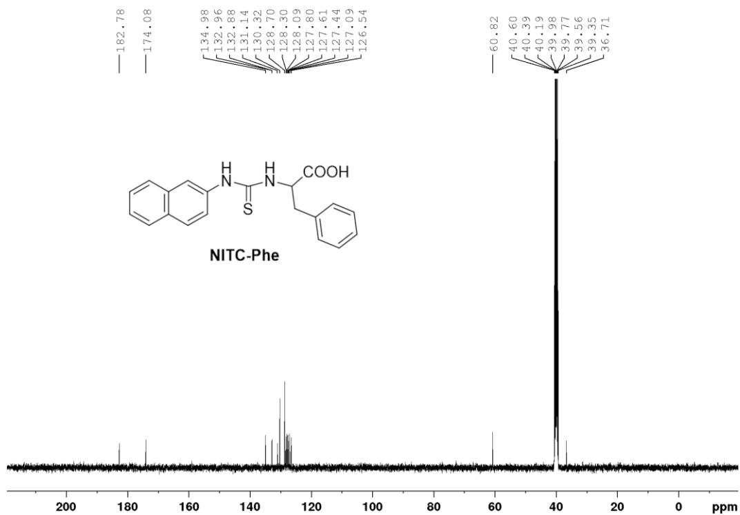
Fig. S31 ^{13}\text{C} NMR spectrum of NITC-Phe.
