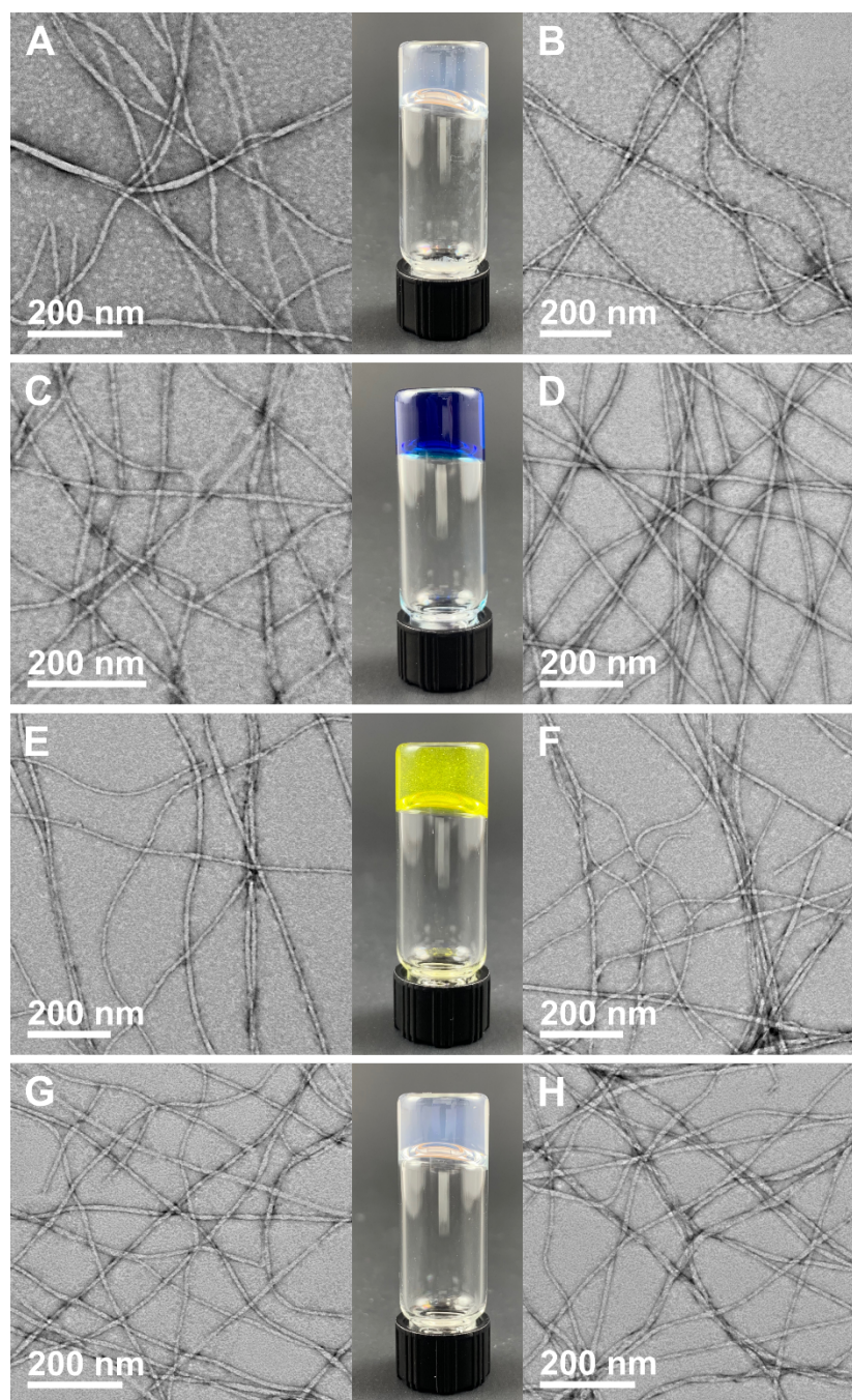
Figure S10. TEM images of hydrogels of 1b one and five days after triggering gelation, and digital image of hydrogels after one day (no change was observed after five days). (A–B) Unloaded hydrogel after (A) one day and (B) five days. (C–D) Hydrogel loaded with methylene blue after (A) one day and (B) five days. (E–F) Hydrogel loaded with naphthol yellow S after (E) one day and (F) five days. (G–H) Hydrogel loaded with caffeine after (G) one day and (H) five days.
