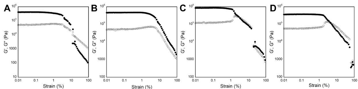
Figure S18. Strain sweep data collected via oscillatory rheology for 20 mM hydrogels of gelator 3b . G' and G'' values (Pa) are represented by closed circles and open circles, respectively. (A) Unloaded hydrogel. (B) Hydrogel loaded with methylene blue. (C) Hydrogel loaded with naphthol yellow S. (D) Hydrogel loaded with caffeine.
