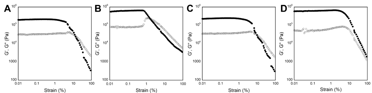
Figure S17. Strain sweep data collected via oscillatory rheology for 20 mM hydrogels of gelator 2b . G' and G'' values (Pa) are represented by closed circles and open circles, respectively. (A) Unloaded hydrogel. (B) Hydrogel loaded with methylene blue. (C) Hydrogel loaded with naphthol yellow S. (D) Hydrogel loaded with caffeine.
