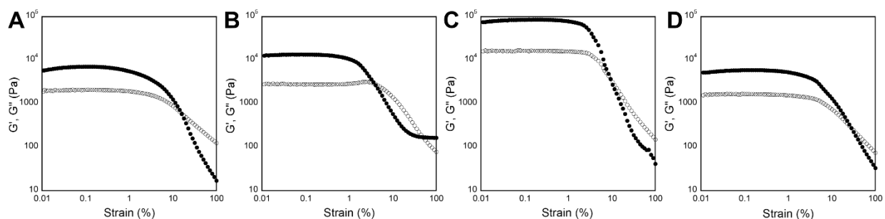
Figure S13. Strain sweep data collected via oscillatory rheology for 20 mM hydrogels of gelator 1a . G' and G'' values (Pa) are represented by closed circles and open circles, respectively. (A) Unloaded hydrogel. (B) Hydrogel loaded with methylene blue. (C) Hydrogel loaded with naphthol yellow S. (D) Hydrogel loaded with caffeine.
