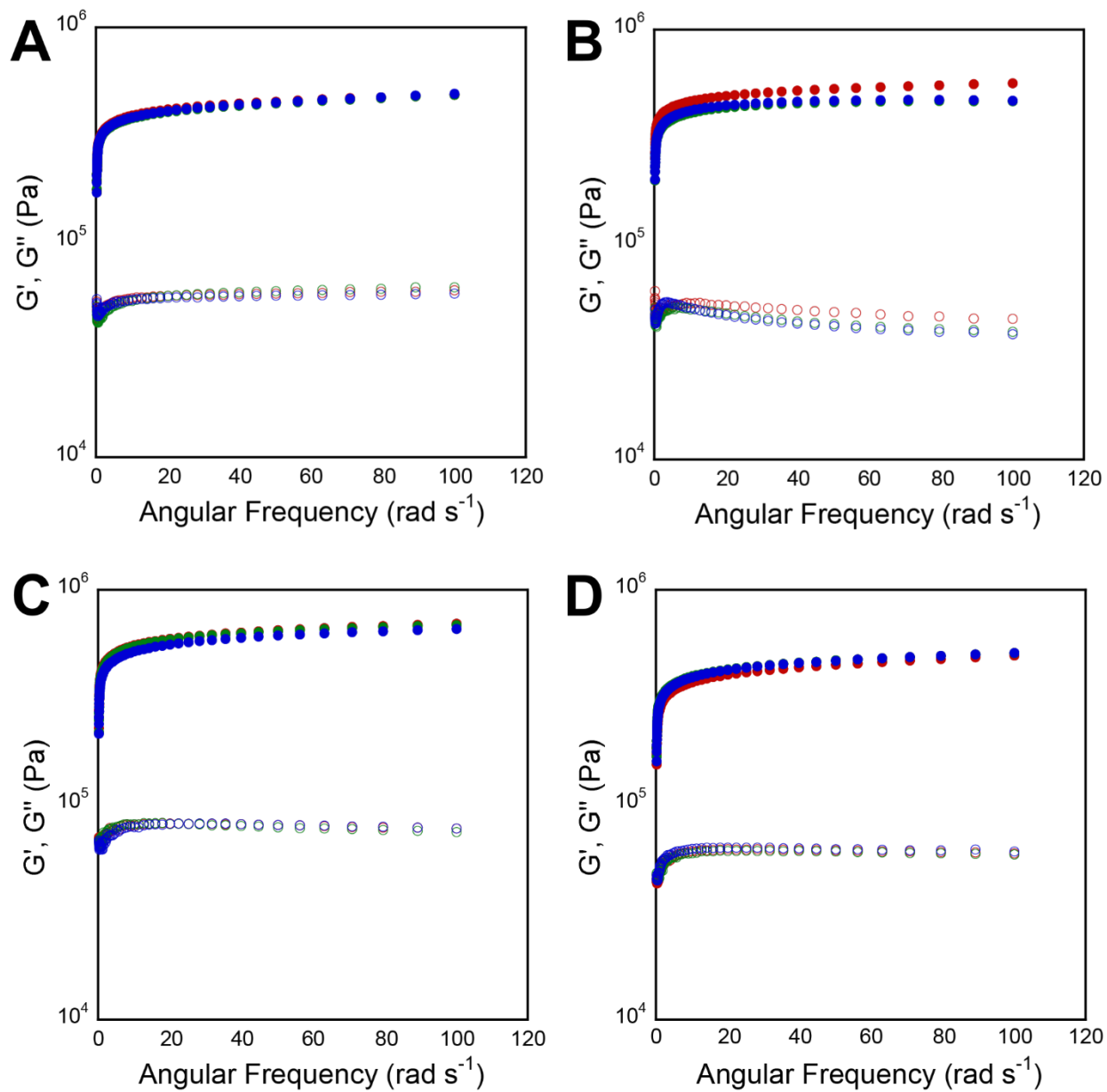
Figure S24. Frequency sweep data collected via oscillatory rheology for 20 mM hydrogels of gelator 3b . G' and G'' values (Pa) are represented by closed circles and open circles, respectively. Each plot contains three distinct measurements of three separate hydrogels. (A) Unloaded hydrogel. (B) Hydrogel loaded with methylene blue. (C) Hydrogel loaded with naphthol yellow S. (D) Hydrogel loaded with caffeine.
