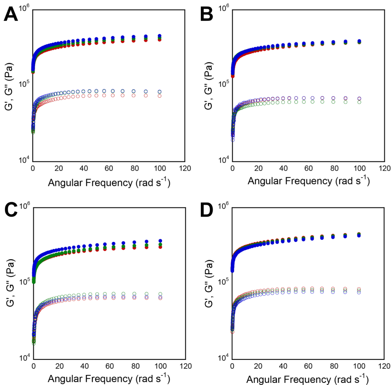
Figure S20. Frequency sweep data collected via oscillatory rheology for 20 mM hydrogels of gelator 2a . G' and G'' values (Pa) are represented by closed circles and open circles, respectively. Each plot contains three distinct measurements of three separate hydrogels. (A) Unloaded hydrogel. (B) Hydrogel loaded with methylene blue. (C) Hydrogel loaded with naphthol yellow S. (D) Hydrogel loaded with caffeine.
