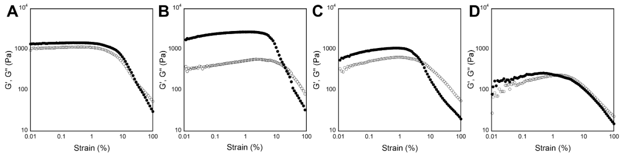
Figure S16. Strain sweep data collected via oscillatory rheology for 20 mM hydrogels of gelator 1b . G' and G'' values (Pa) are represented by closed circles and open circles, respectively. (A) Unloaded hydrogel. (B) Hydrogel loaded with methylene blue. (C) Hydrogel loaded with naphthol yellow S. (D) Hydrogel loaded with caffeine.
