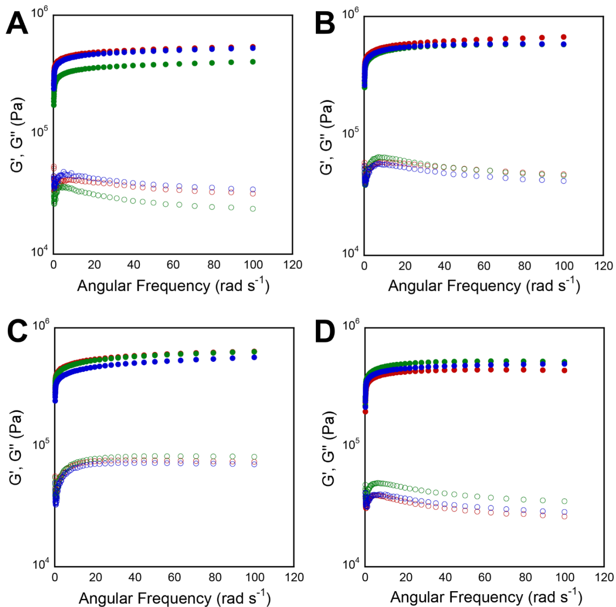
Figure S23. Frequency sweep data collected via oscillatory rheology for 20 mM hydrogels of gelator 2b . G' and G'' values (Pa) are represented by closed circles and open circles, respectively. Each plot contains three distinct measurements of three separate hydrogels. (A) Unloaded hydrogel. (B) Hydrogel loaded with methylene blue. (C) Hydrogel loaded with naphthol yellow S. (D) Hydrogel loaded with caffeine.
