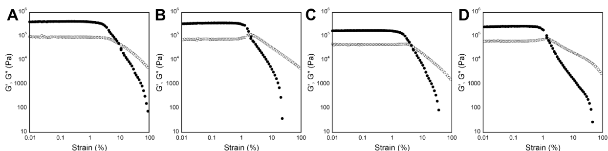
Figure S14. Strain sweep data collected via oscillatory rheology for 20 mM hydrogels of gelator 2a . G' and G'' values (Pa) are represented by closed circles and open circles, respectively. (A) Unloaded hydrogel. (B) Hydrogel loaded with methylene blue. (C) Hydrogel loaded with naphthol yellow S. (D) Hydrogel loaded with caffeine.
