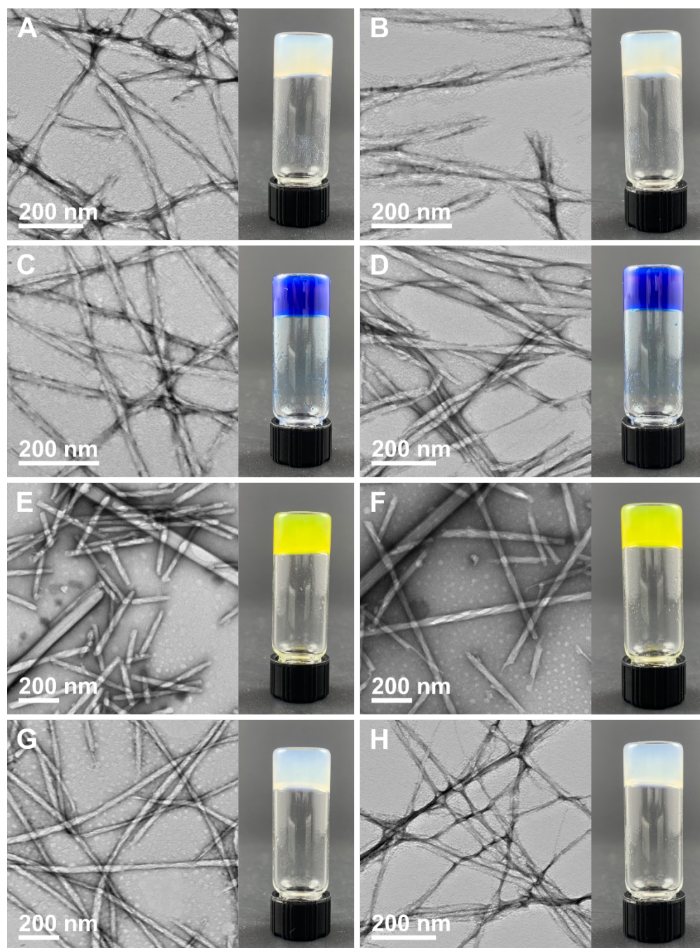
Figure S9. TEM and digital images of hydrogels of 3a one and five days after triggering gelation. (A–B) Unloaded hydrogel after (A) one day and (B) five days. (C–D) Hydrogel loaded with methylene blue after (A) one day and (B) five days. (E–F) Hydrogel loaded with naphthol yellow S after (E) one day and (F) five days. (G–H) Hydrogel loaded with caffeine after (G) one day and (H) five days.
