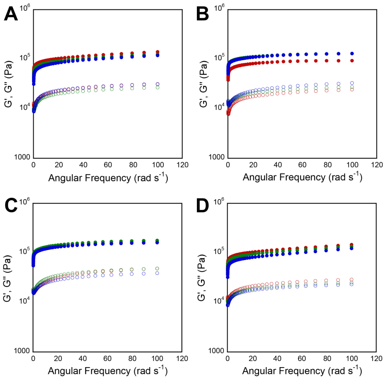
Figure S21. Frequency sweep data collected via oscillatory rheology for 20 mM hydrogels of gelator 3a . G' and G'' values (Pa) are represented by closed circles and open circles, respectively. Each plot contains three distinct measurements of three separate hydrogels. (A) Unloaded hydrogel. (B) Hydrogel loaded with methylene blue. (C) Hydrogel loaded with naphthol yellow S. (D) Hydrogel loaded with caffeine.
