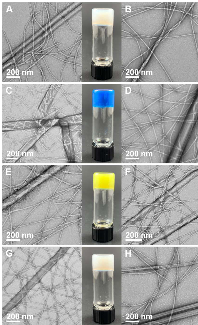
Figure S12. TEM images of hydrogels of 3b one and five days after triggering gelation, and digital image of hydrogels after one day (no change was observed after five days). (A–B) Unloaded hydrogel after (A) one day and (B) five days. (C–D) Hydrogel loaded with methylene blue after (A) one day and (B) five days. (E–F) Hydrogel loaded with naphthol yellow S after (E) one day and (F) five days. (G–H) Hydrogel loaded with caffeine after (G) one day and (H) five days.
