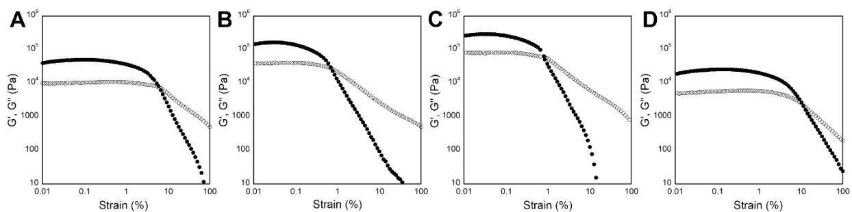
Figure S15. Strain sweep data collected via oscillatory rheology for 20 mM hydrogels of gelator 3a . G' and G'' values (Pa) are represented by closed circles and open circles, respectively. (A) Unloaded hydrogel. (B) Hydrogel loaded with methylene blue. (C) Hydrogel loaded with naphthol yellow S. (D) Hydrogel loaded with caffeine.
