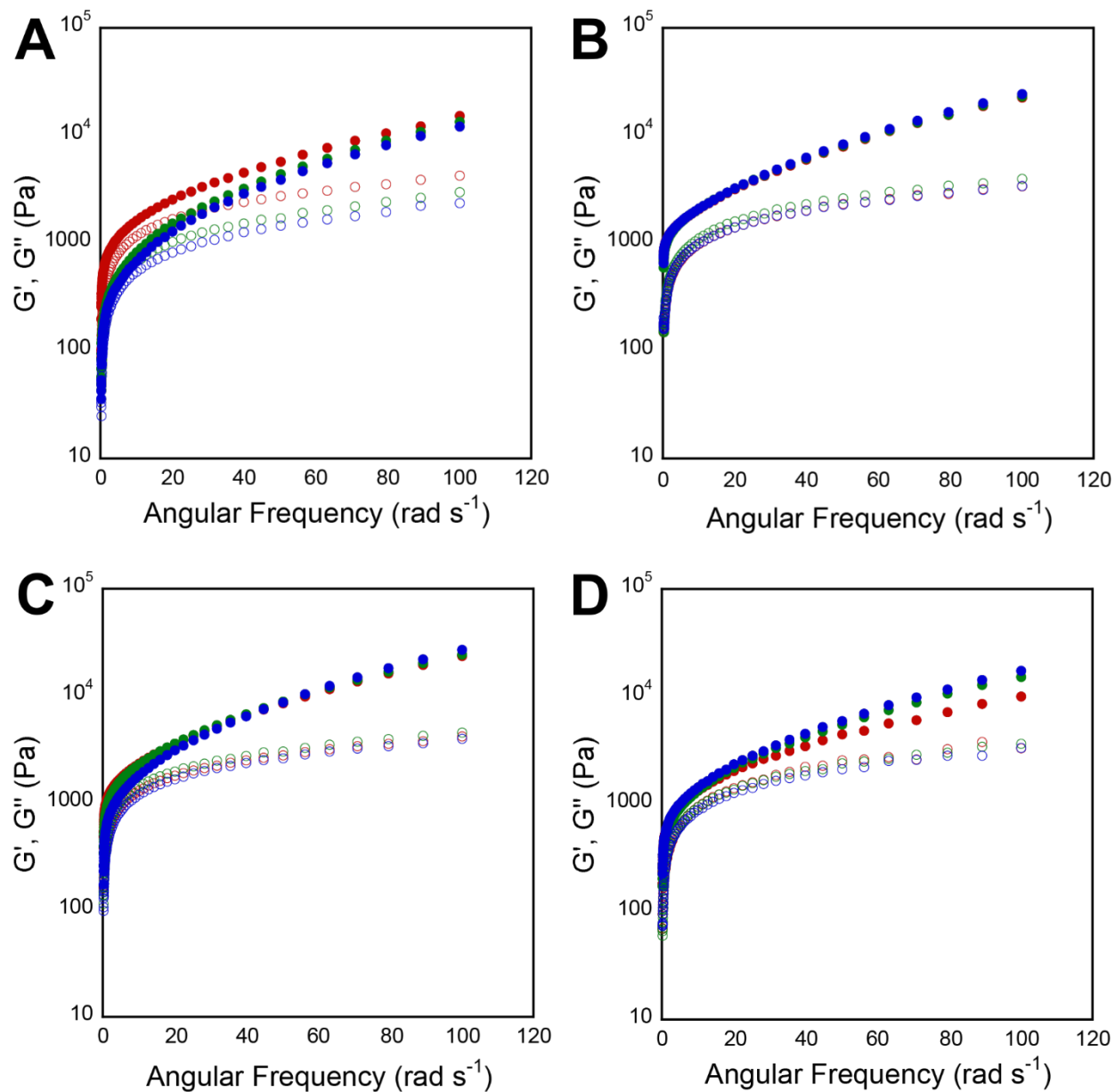
Figure S22. Frequency sweep data collected via oscillatory rheology for 20 mM hydrogels of gelator 1b . G' and G'' values (Pa) are represented by closed circles and open circles, respectively. Each plot contains three distinct measurements of three separate hydrogels. (A) Unloaded hydrogel. (B) Hydrogel loaded with methylene blue. (C) Hydrogel loaded with naphthol yellow S. (D) Hydrogel loaded with caffeine.
