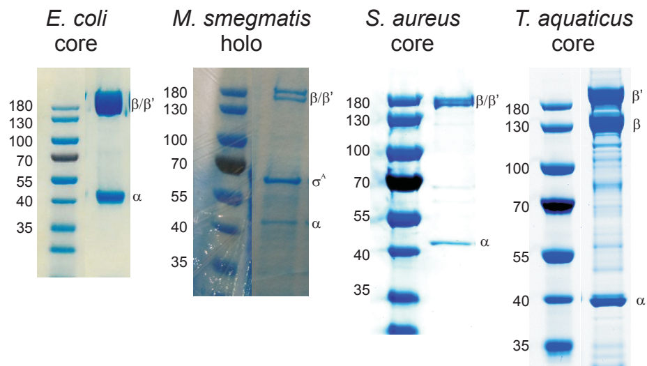
Figure S1. SDS-gels of the purified RNAP core and holoenzymes. Left lane in each gel is a size marker.
