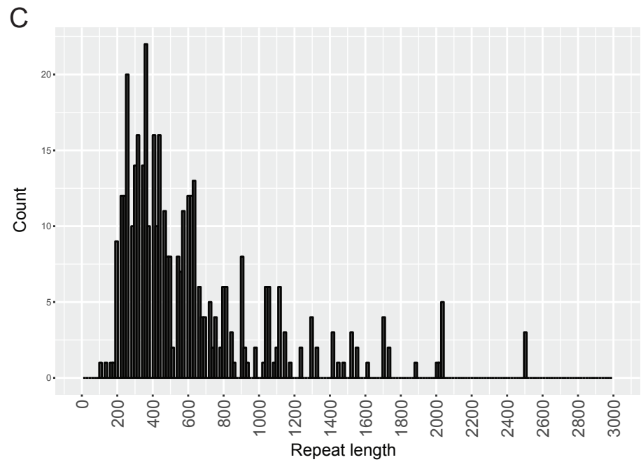
Supplementary Fig. S4 Sequence analysis of GA-rich regions Long hits (without genes) n=435, A) G and C content and B) GA content. C) GA region length of regions present in long hits n=409. 14 hits not included on graph (>3000 bp). D) Genomic GA regions (n=10266) replicated at the time of labelling (n=3802).
