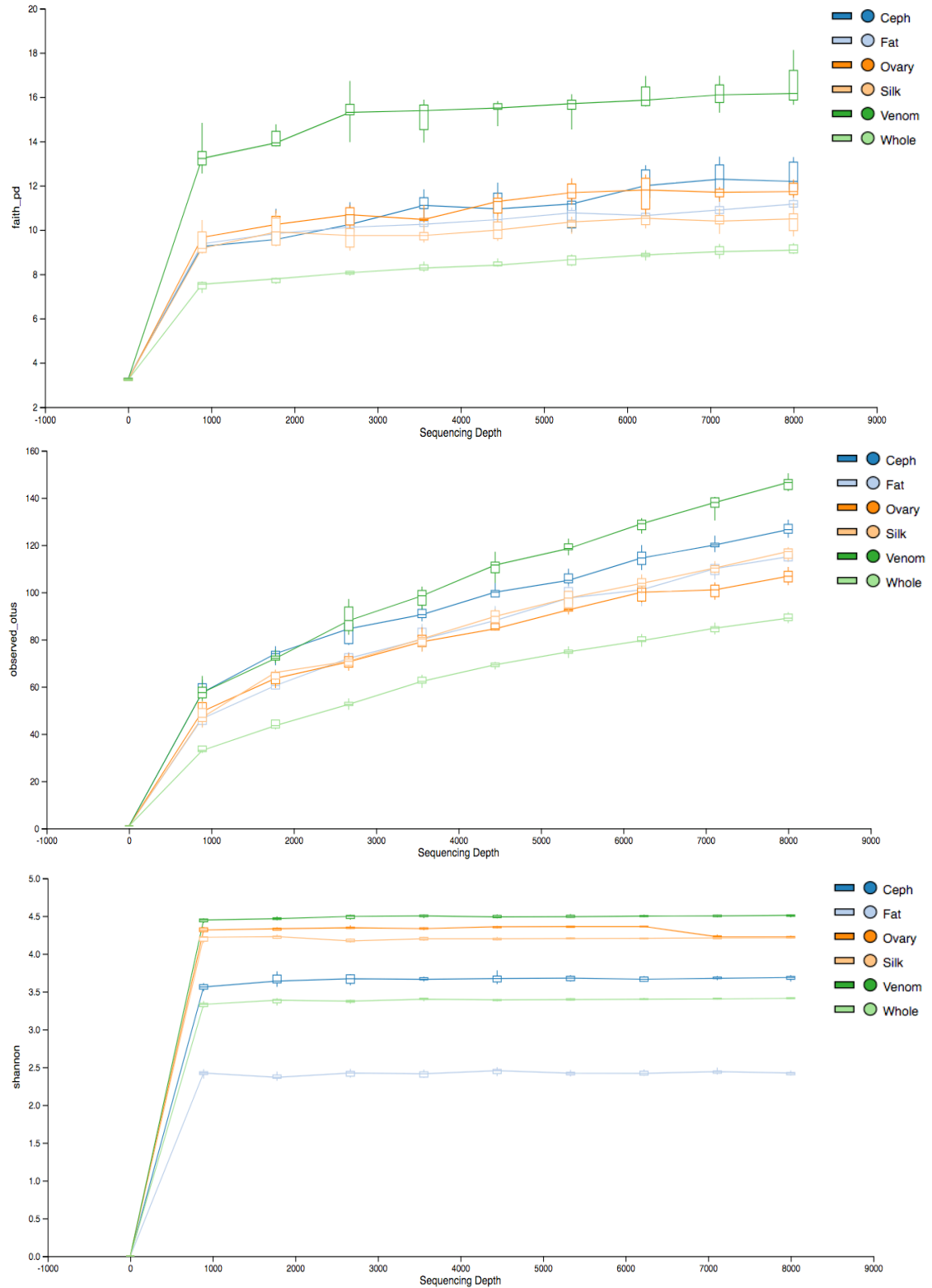
Figure S2. QIIME 2 Microbial Alpha-Diversity Plots. Alpha-Rarefaction results for Faith-PD (a), Observed OTUs (b), and Shannon Index (c) with Depth of Coverage at 8,000 rarified sequences.
