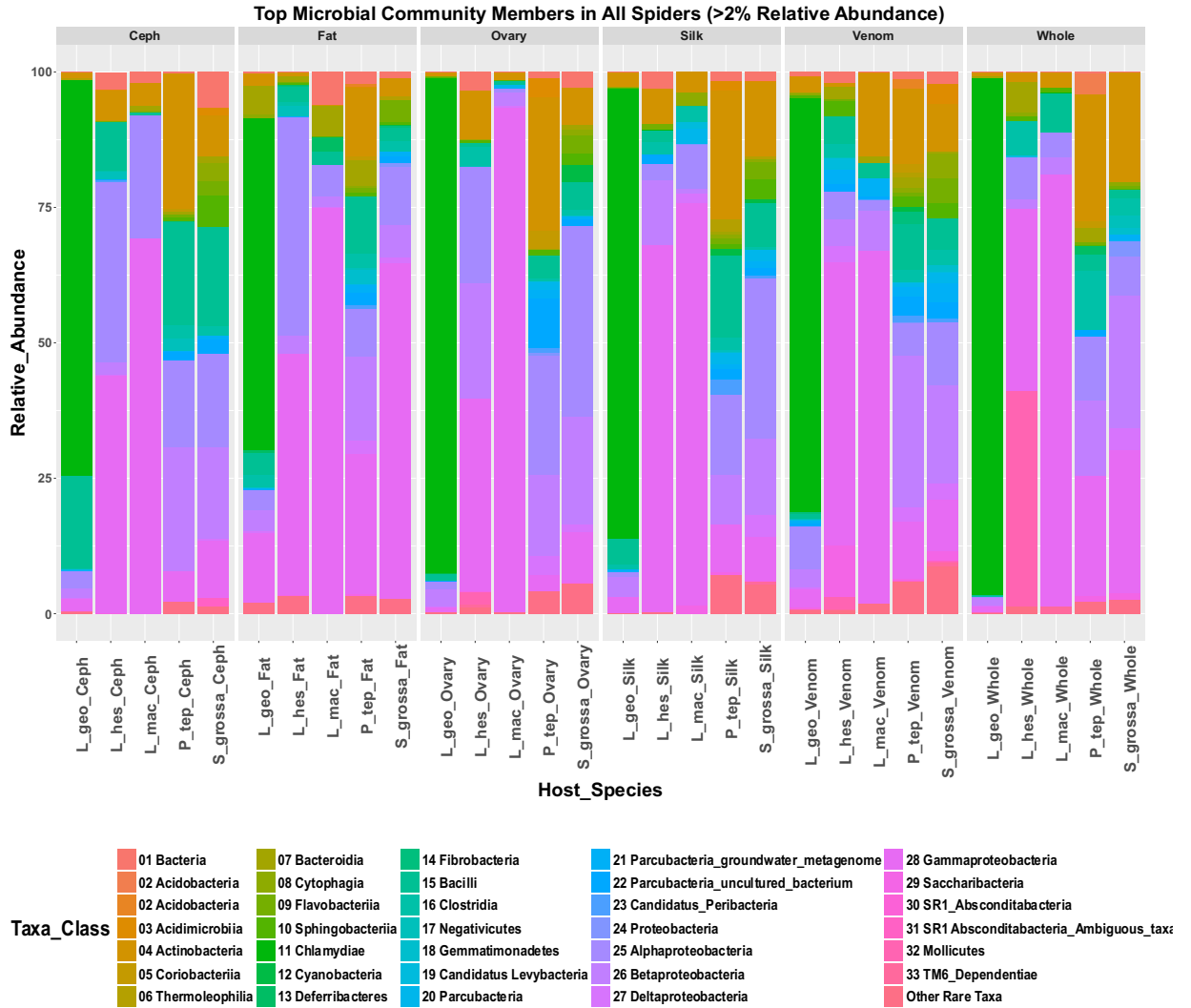
Figure S3. Taxa Plots per Tissue Type – Level 3, Class. Major microbial constituents by class (>2%) within each whole spider and tissue sample for each species (replicates grouped via mean-ceiling). Sample types as follows: Whole Spiders, Cephalothorax, Venom Glands, Ovary, Silk Glands, and Fat Tissue.
