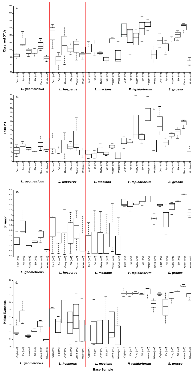
Figure S4. QIIME 2 Alpha Diversity Group Significance Testing. Box plots of alpha diversity tests grouped by base sample type. Overall Kruskal-Wallis p-value = 0.00028 (for all groups). (a) Observed OTUs, (b) Faith Phylogenetic-Diversity Index, (c) Shannon Index, (d) Pielou Evenness Index.
