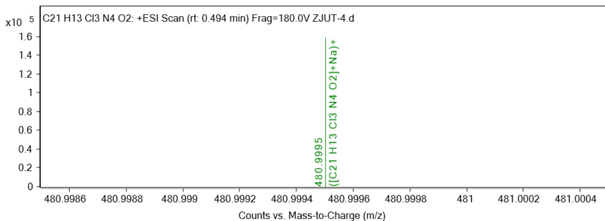
Figure S32 ESI-HRMS spectra of 7d
