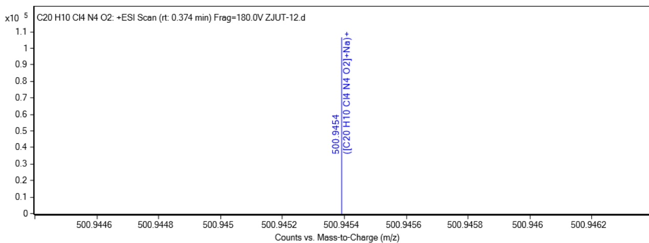
Figure S40 ESI-HRMS spectra of 7l
