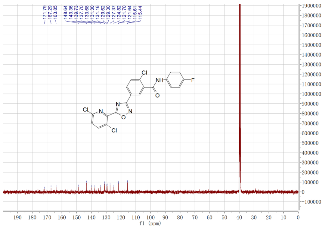
Figure S24 ^{13}\text{C} NMR spectra of 7j
