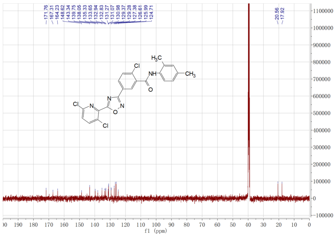
Figure S21 ^{13}\text{C} NMR spectra of 7g
