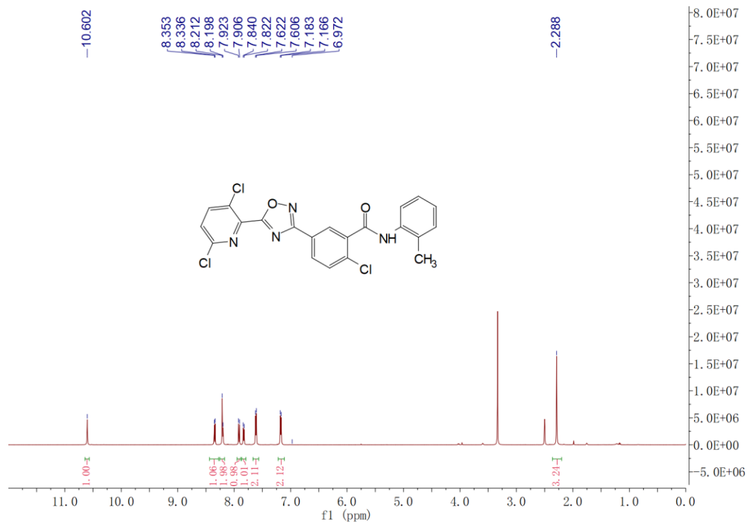
Figure S2 1 H NMR spectra of 7b
