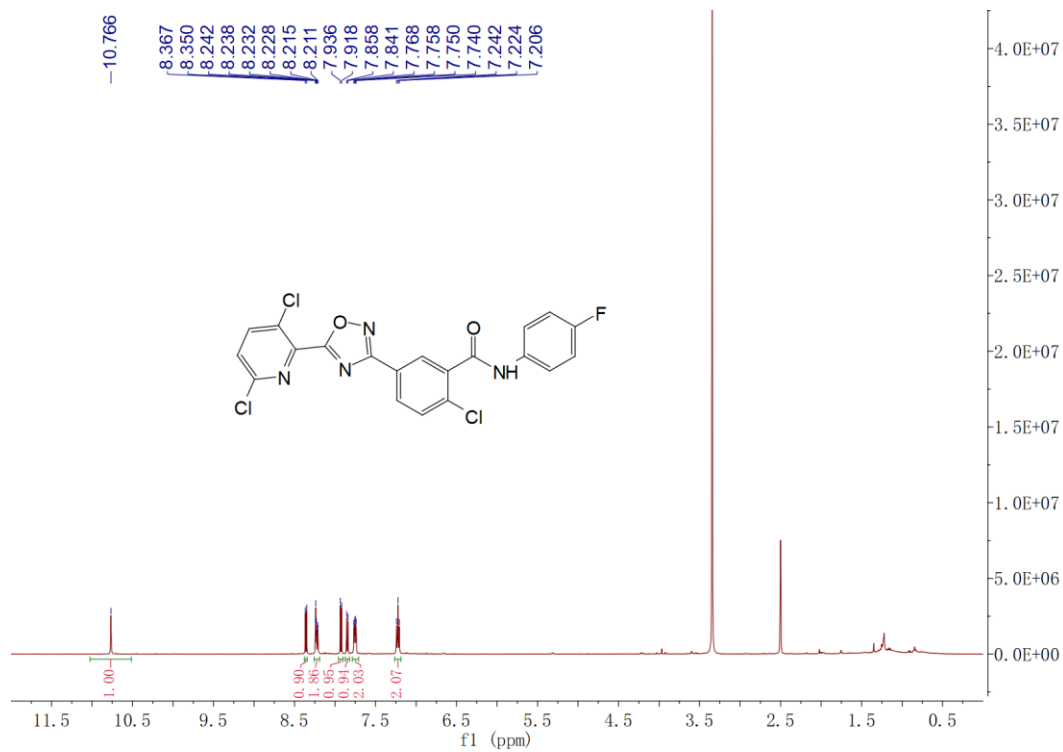
Figure S10 ^1\text{H} NMR spectra of 7j
