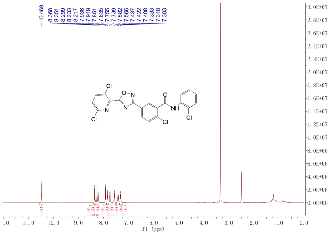
Figure S11 1 H NMR spectra of 7k
