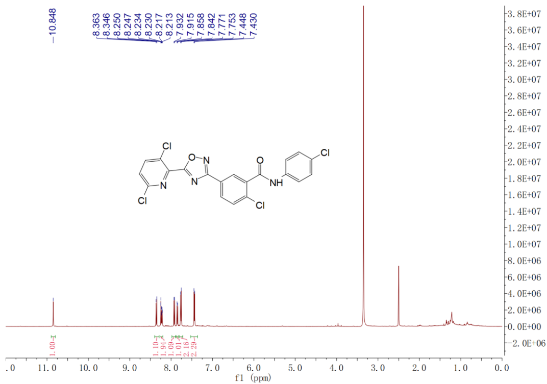
Figure S13 1 H NMR spectra of 7m
