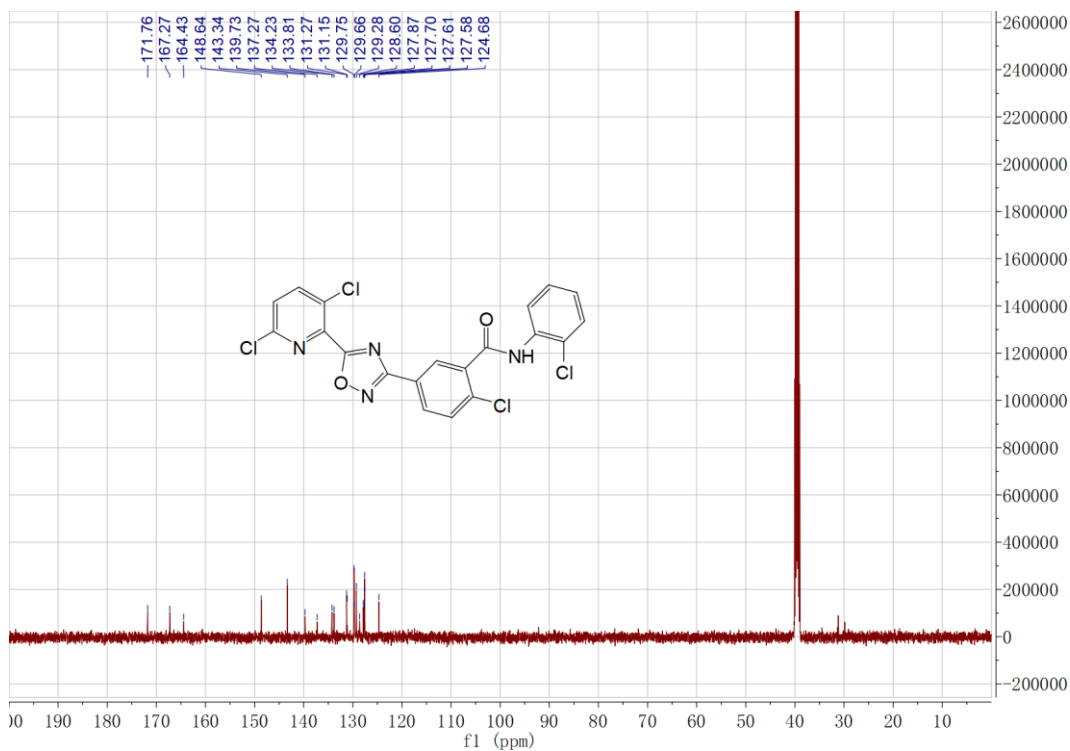
Figure S25 ^{13}\text{C} NMR spectra of 7k
