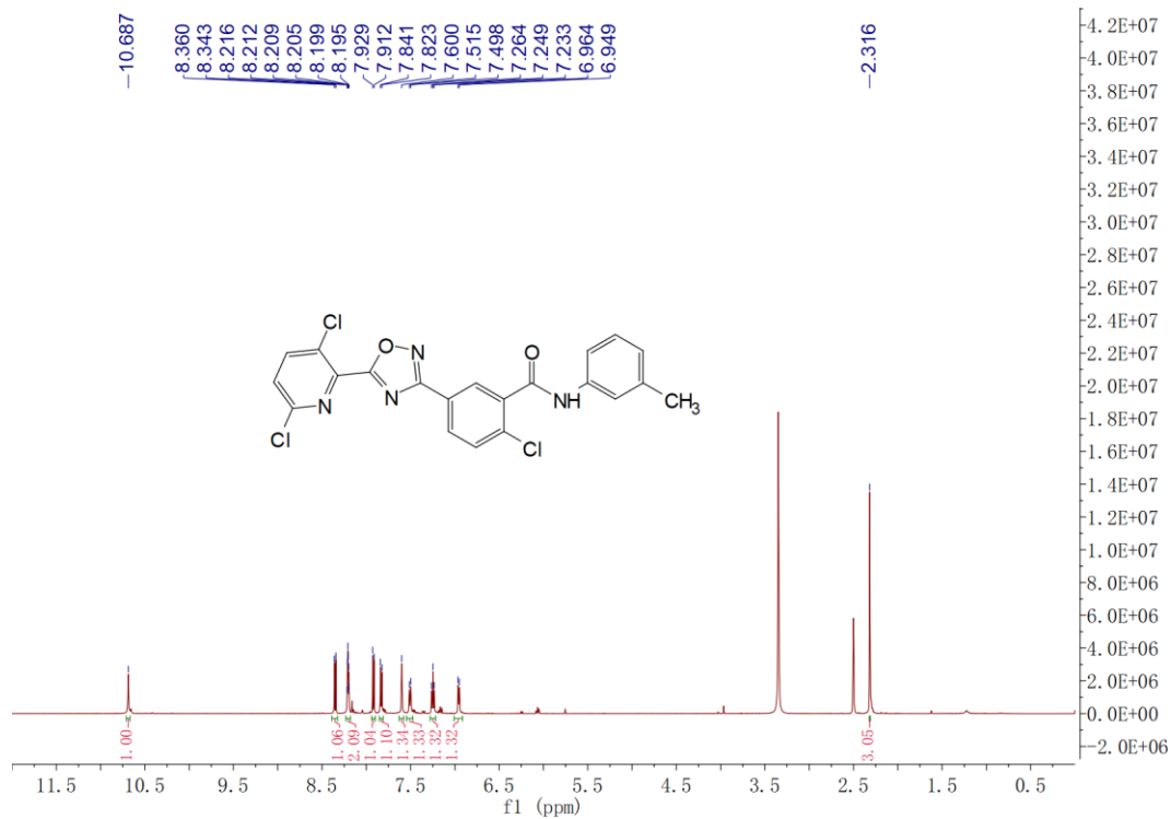
Figure S3 ^1\text{H} NMR spectra of 7c
