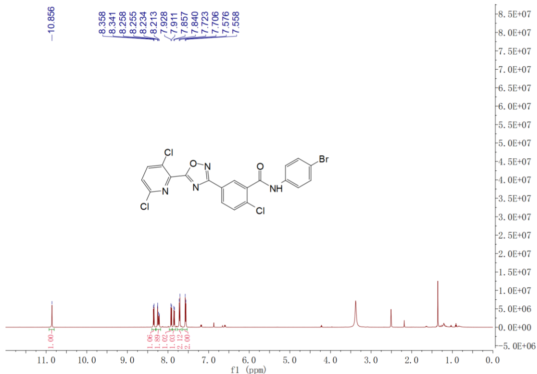
Figure S14 1 H NMR spectra of 7n
