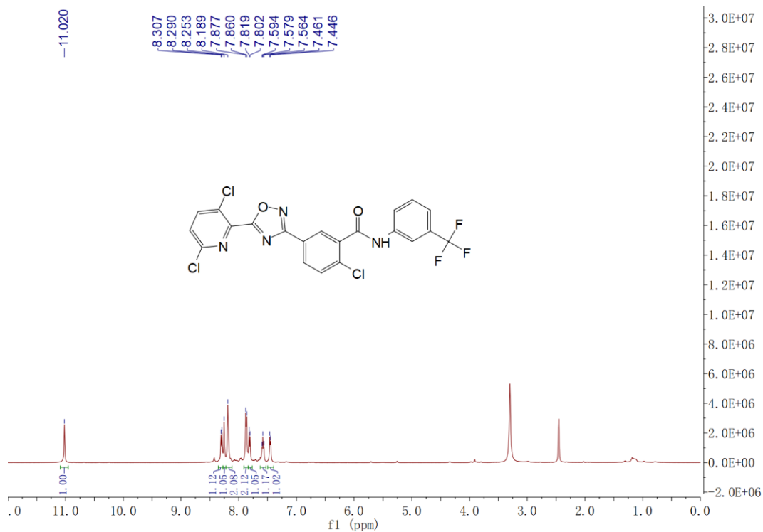
Figure S6 1 H NMR spectra of 7f
