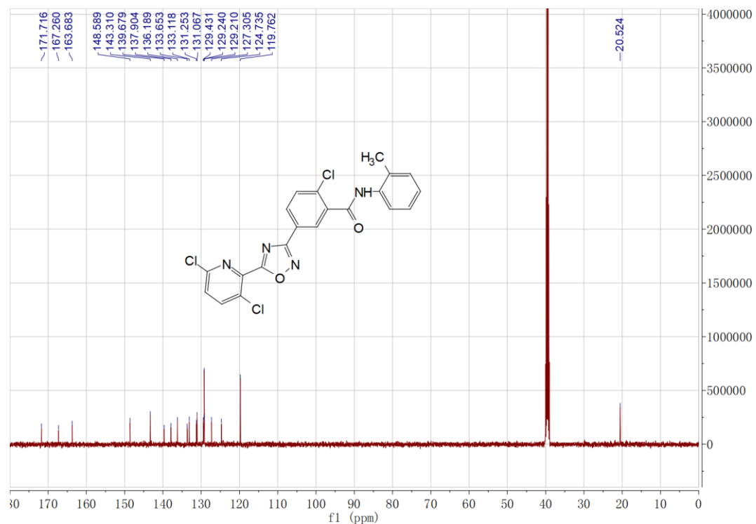
Figure S16 ^{13}\text{C} NMR spectra of 7b
