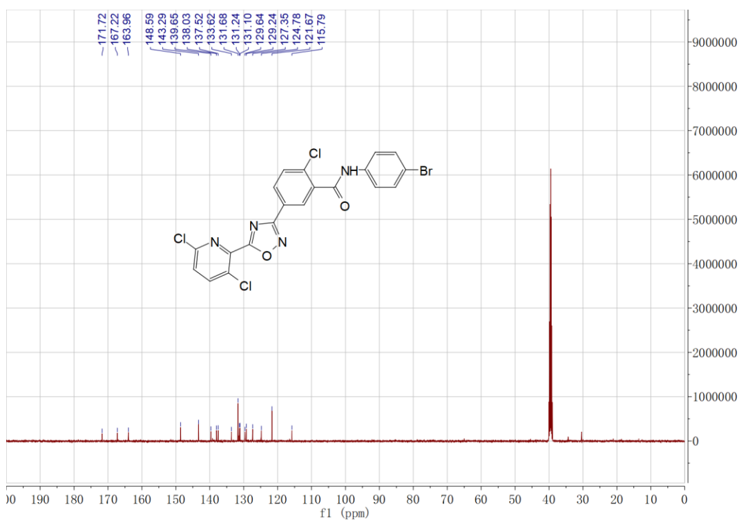
Figure S28 13 C NMR spectra of 7n
