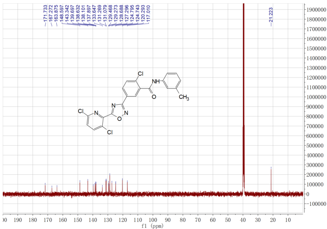
Figure S17 ^{13}\text{C} NMR spectra of 7c
