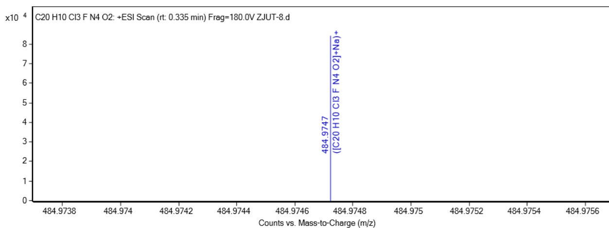
Figure S36 ESI-HRMS spectra of 7h
