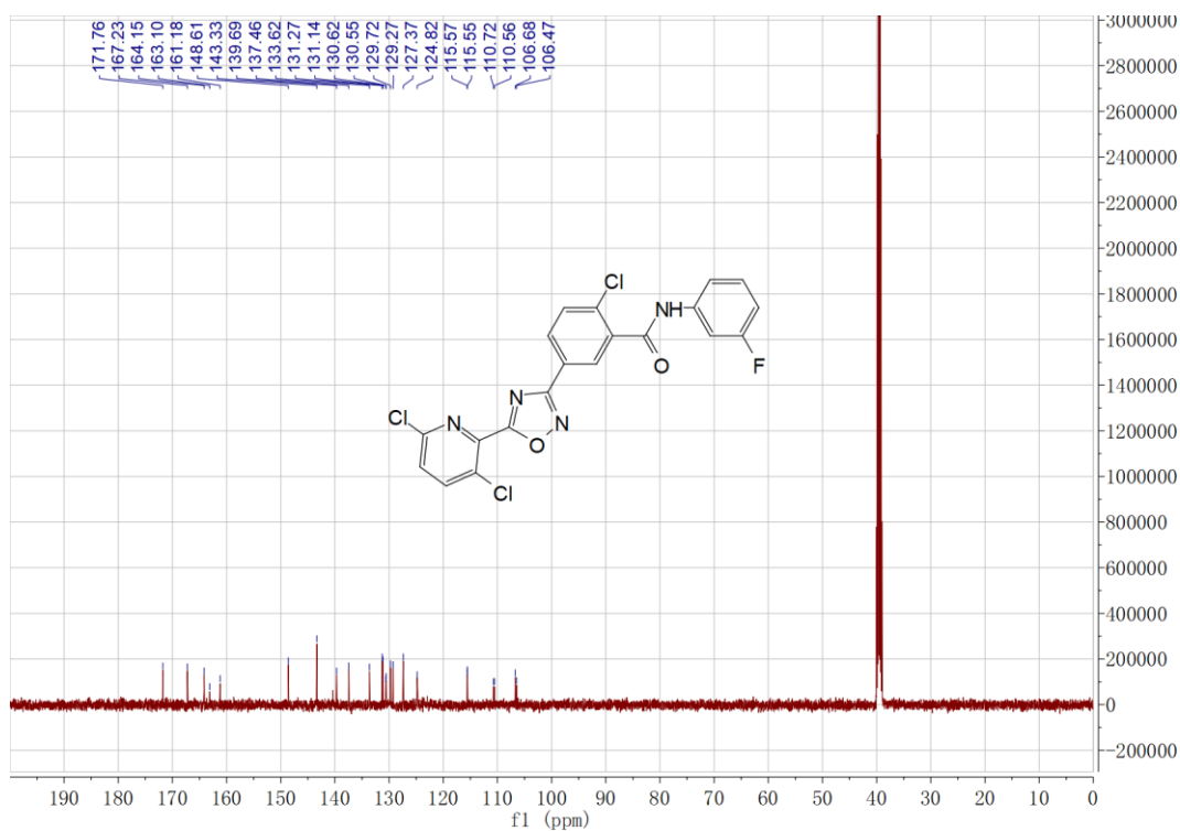
Figure S23 ^{13}\text{C} NMR spectra of 7i
