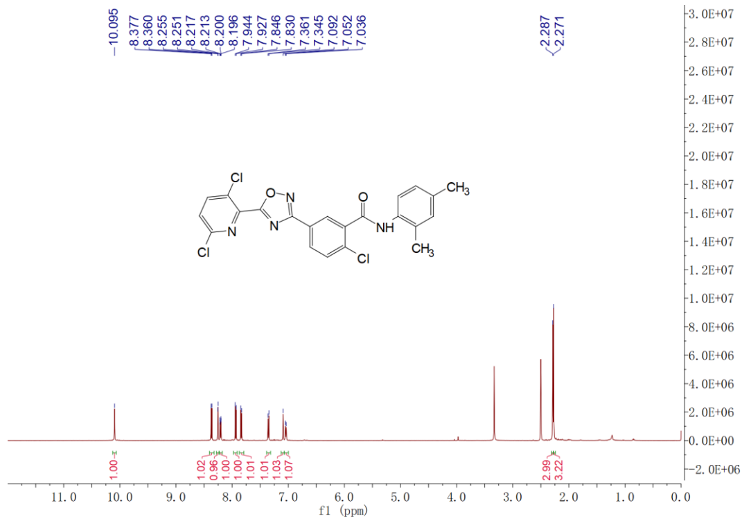
Figure S7 1 H NMR spectra of 7g
