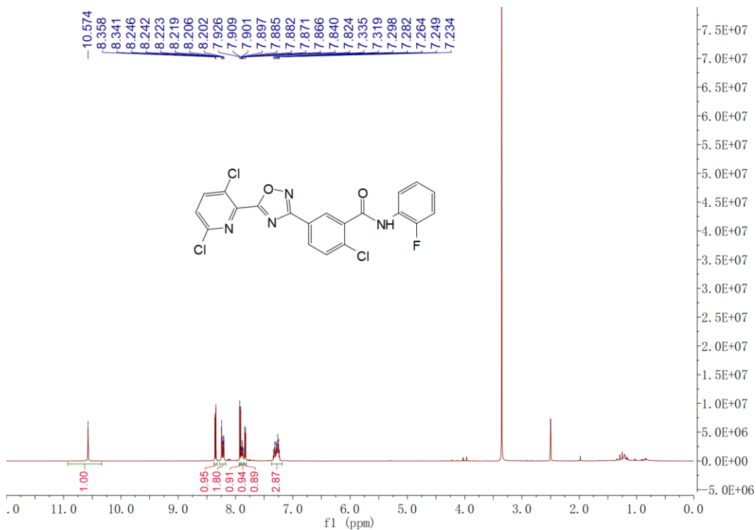
Figure S8 1 H NMR spectra of 7h
