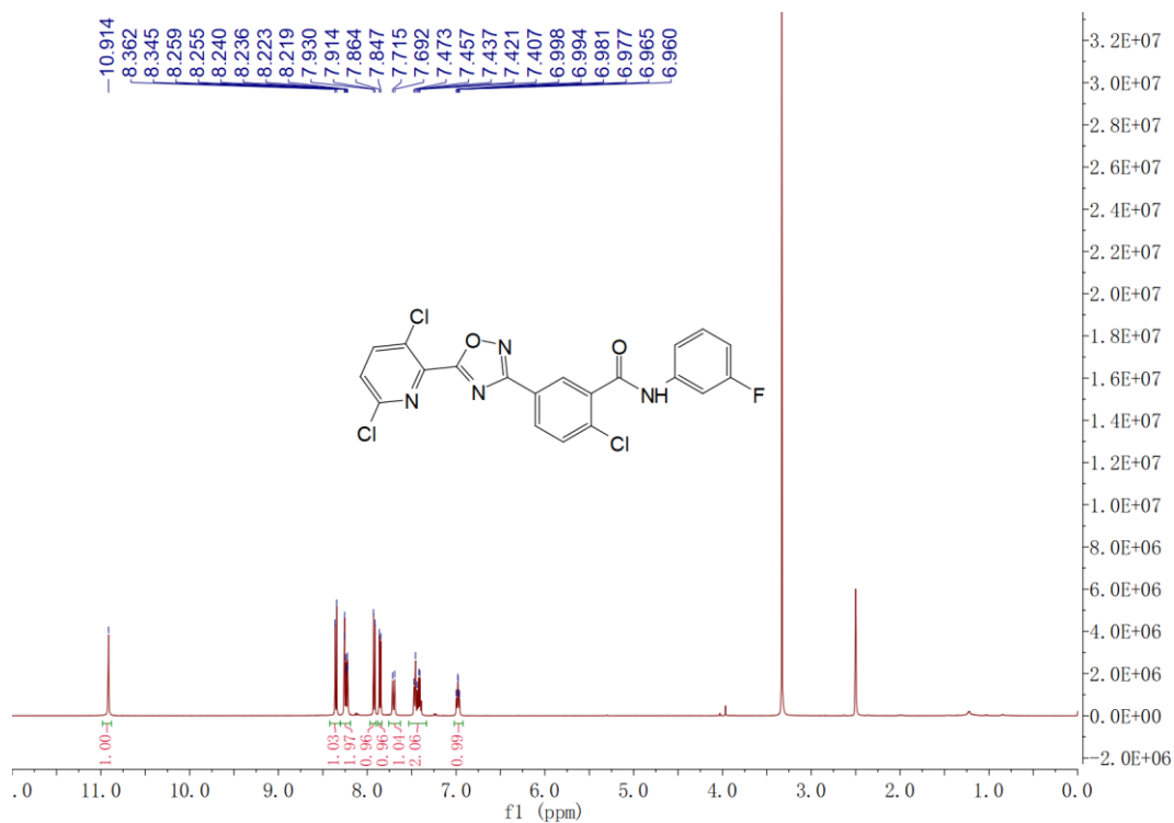
Figure S9 ^1\text{H} NMR spectra of 7i
