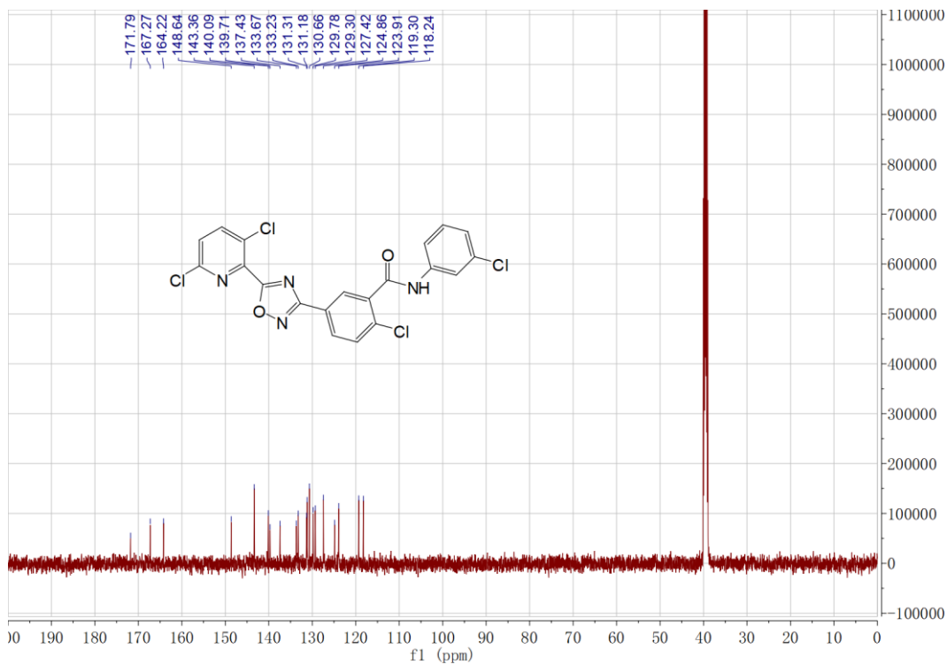
Figure S26 ^{13}\text{C} NMR spectra of 7l
