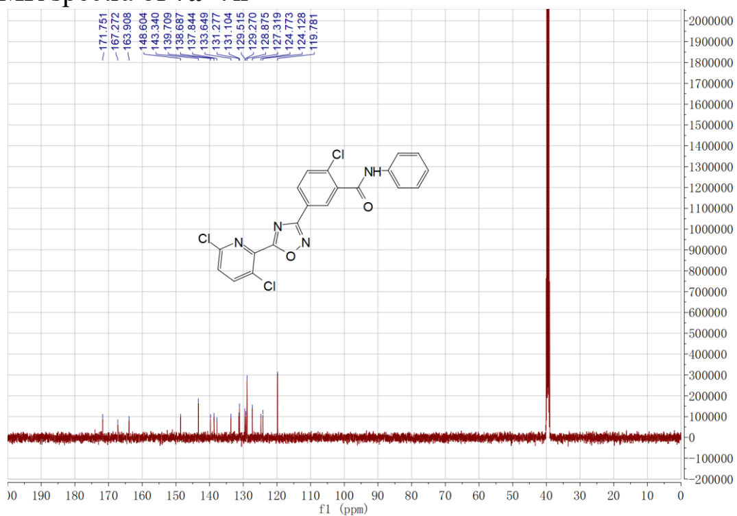
Figure S15 ^{13}\text{C} NMR spectra of 7a
