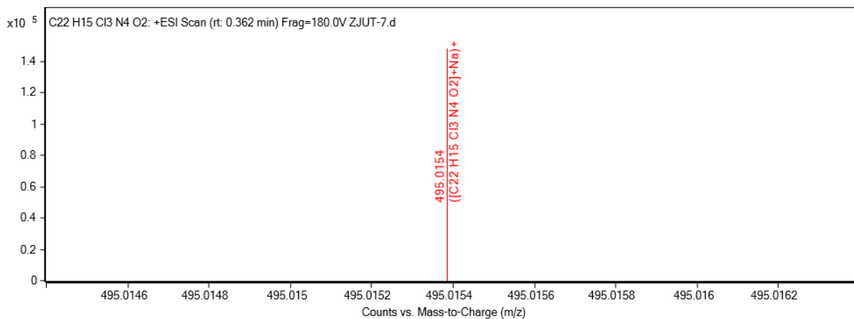
Figure S35 ESI-HRMS spectra of 7g
