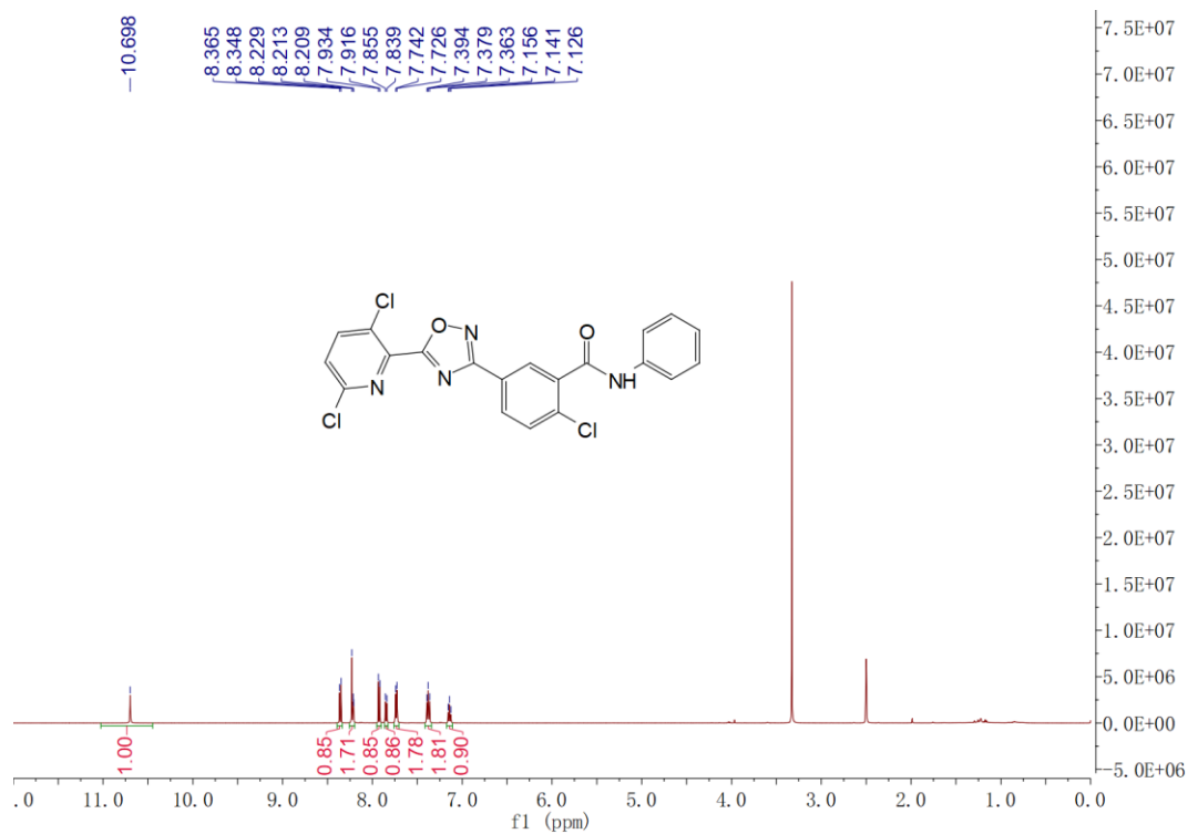
Figure S1 1 H NMR spectra of 7a
