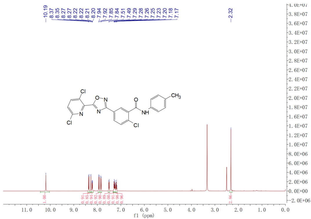
Figure S4 ^1\text{H} NMR spectra of 7d
