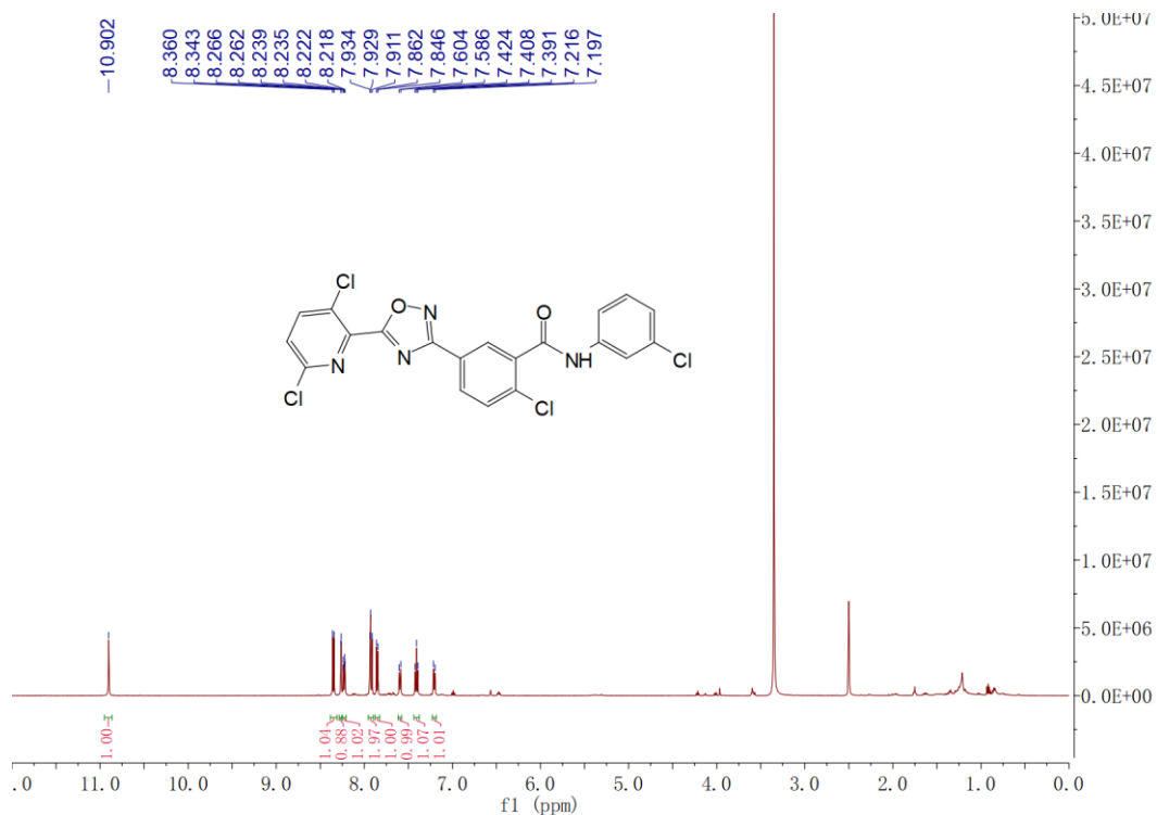
Figure S12 1 H NMR spectra of 7l
