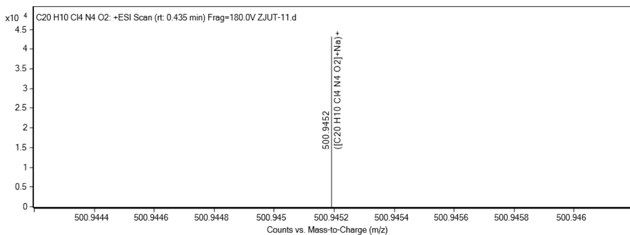
Figure S39 ESI-HRMS spectra of 7k
