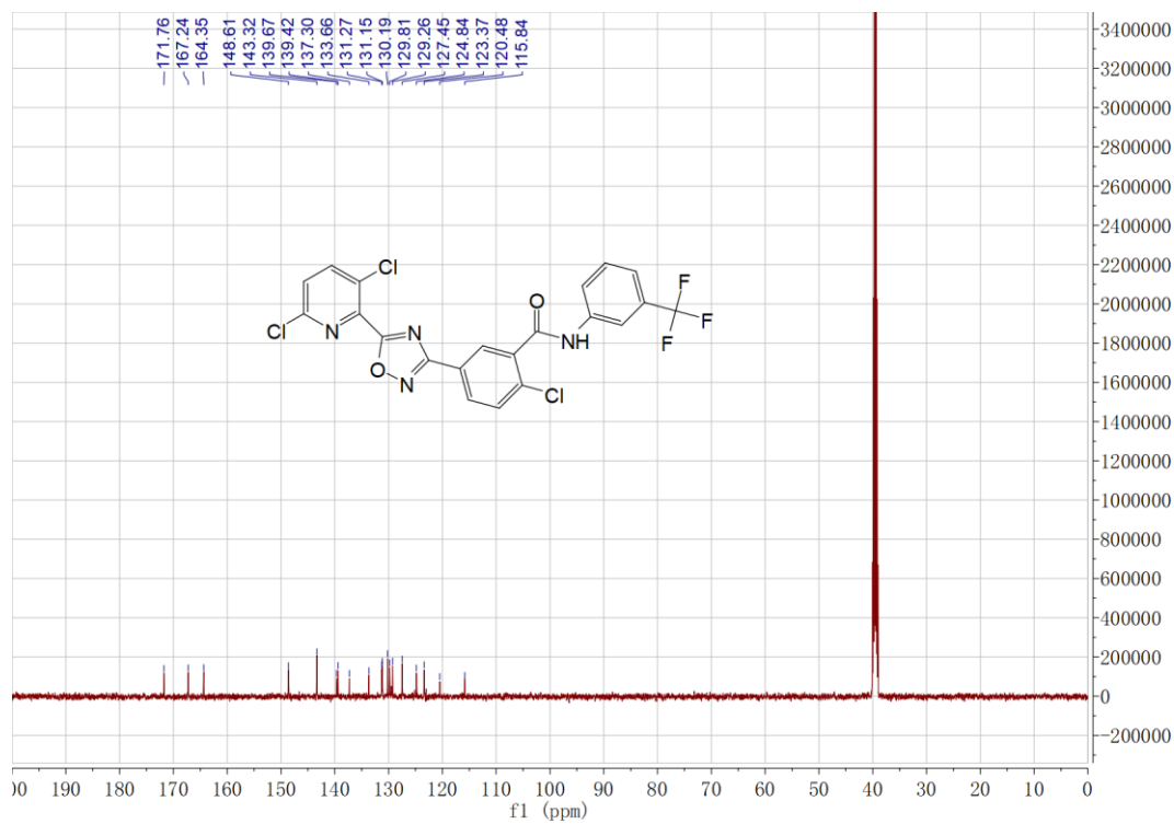
Figure S20 ^{13}\text{C} NMR spectra of 7f
