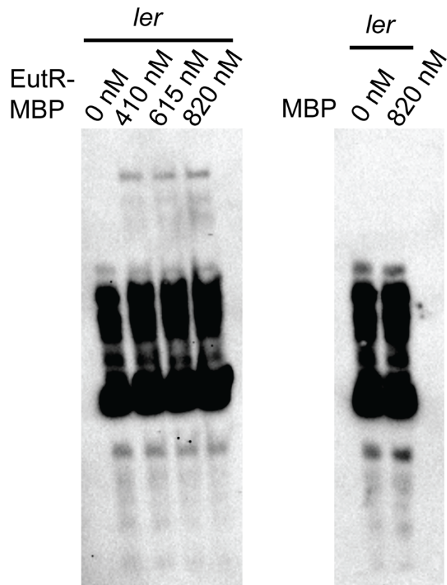
Fig. S3. EMSA of the ler promoter with EutR::MBP or MBP.
