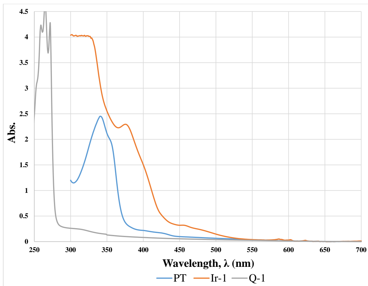
Figure S1: UV-Vis Spectra of the Photocatalysts and HAT Catalyst Used
