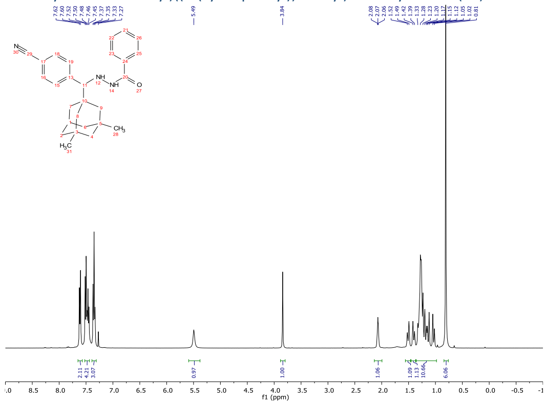
Compound 34 - 1H - 400MHz
