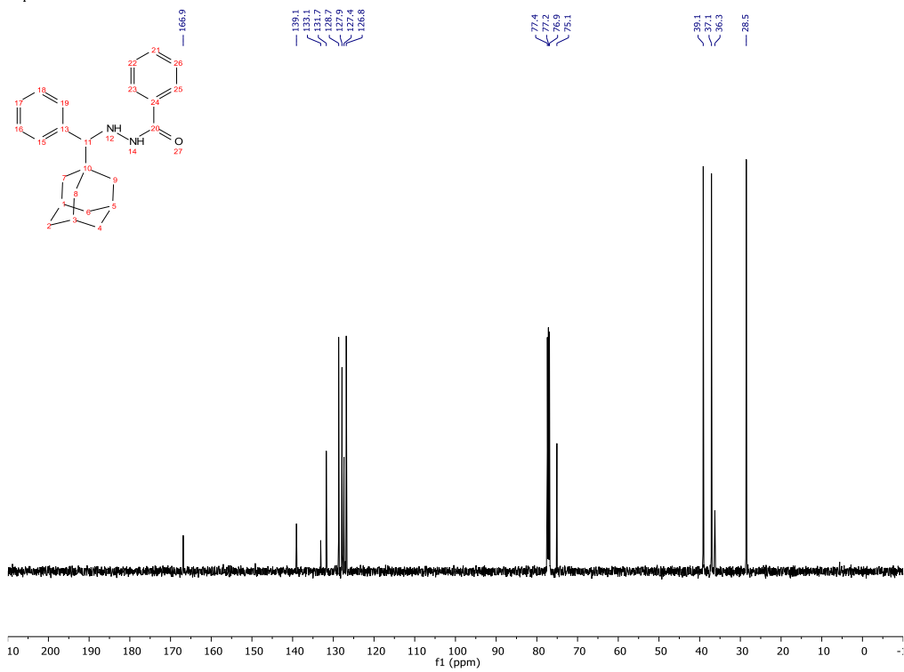
Compound 12 - 13C - 125 MHz
