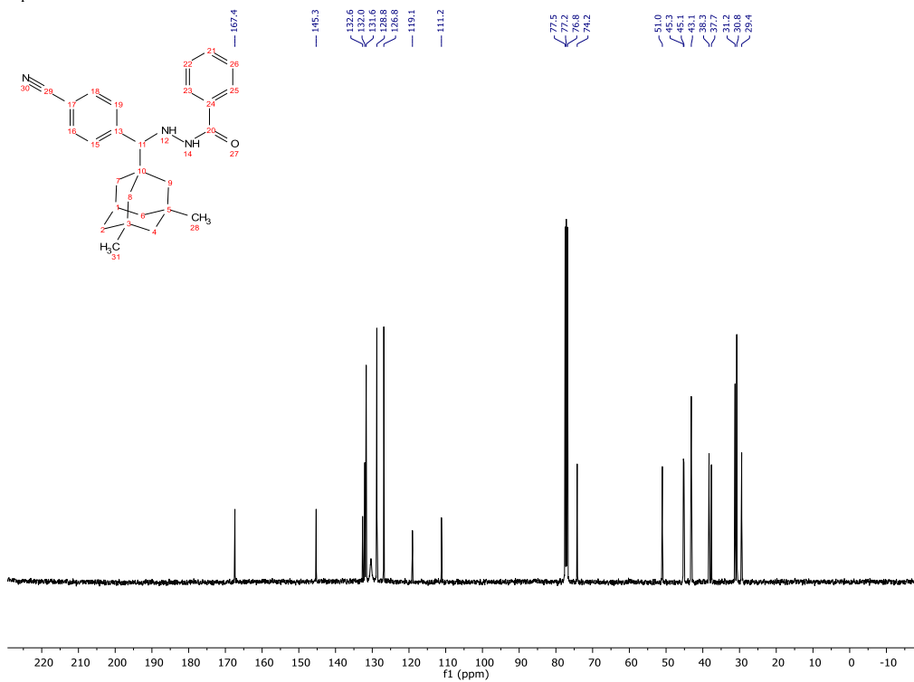
Compound 34 - 13C - 100MHz
