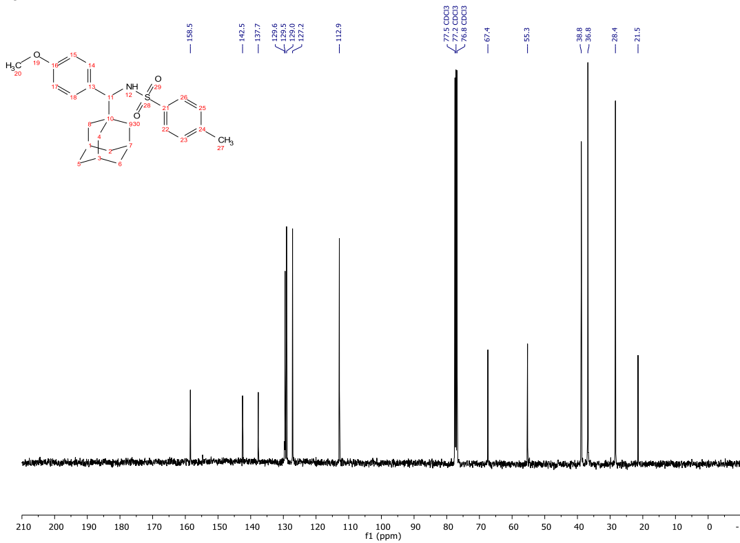
Compound 21 - 13C - 100MHz
