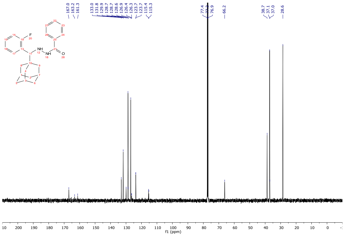
Compound 29 — 13C 125.81 MHz in CDCl 3
