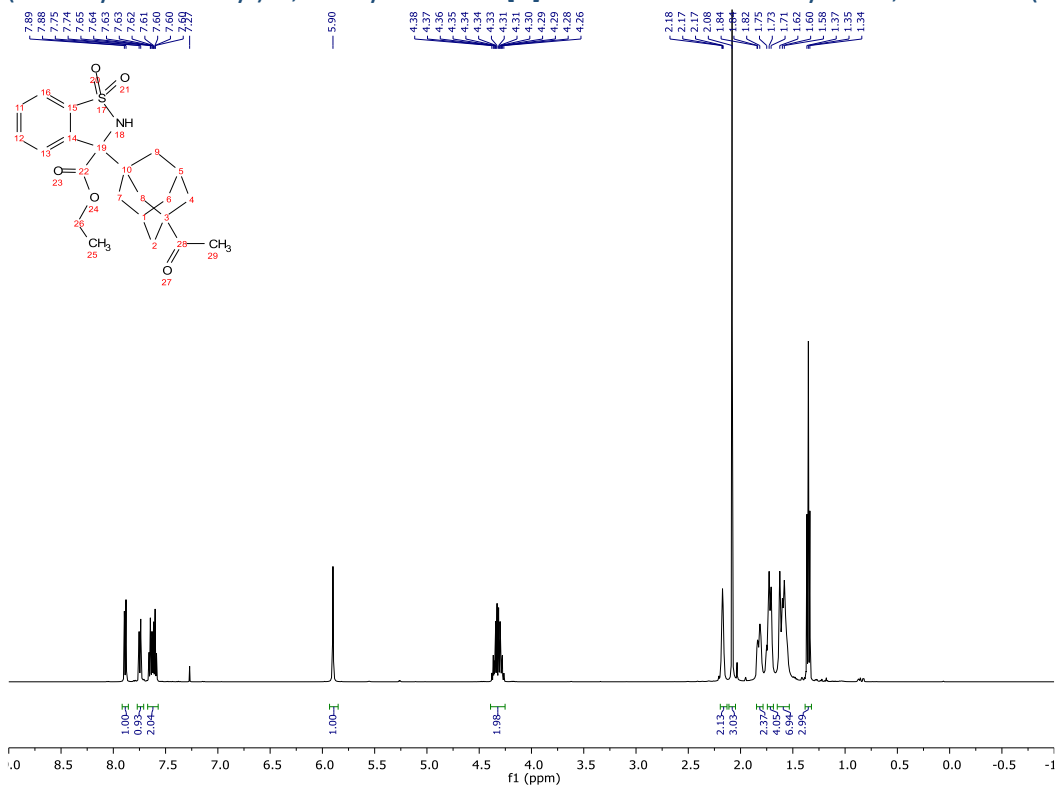
Compound 40 - 1H - 500MHz
