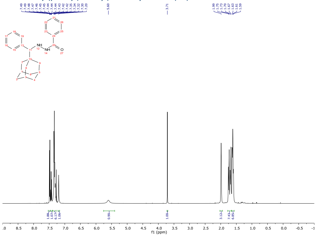
Compound 12 - 1H - 500 MHz
