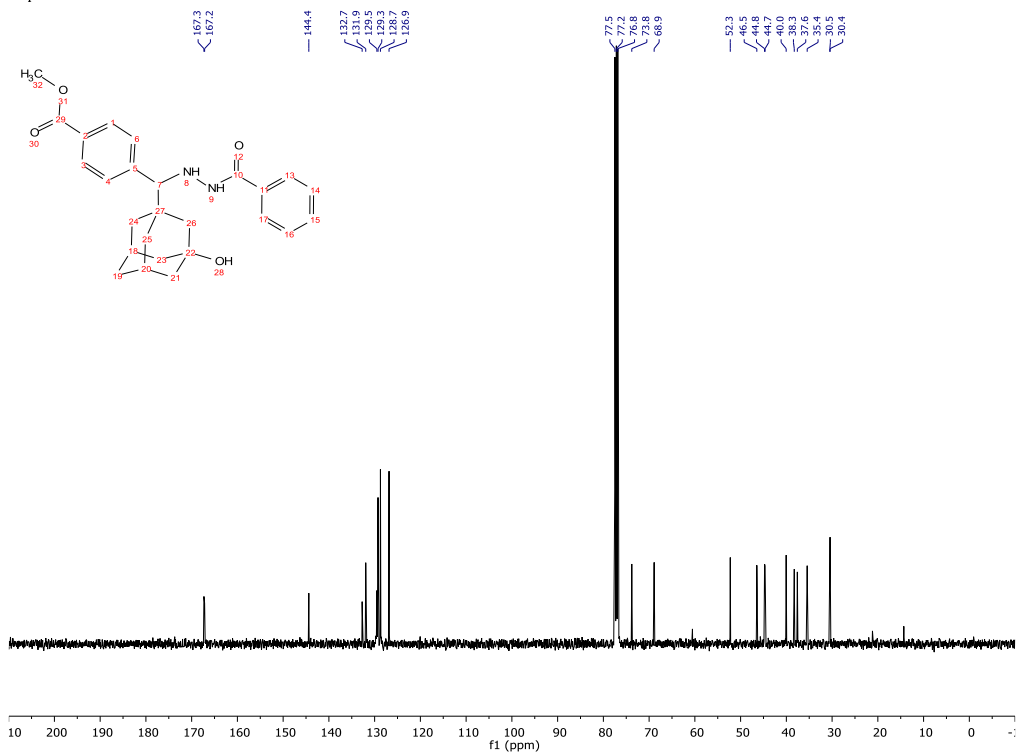
Compound 36 - 13C - 100 MHz
