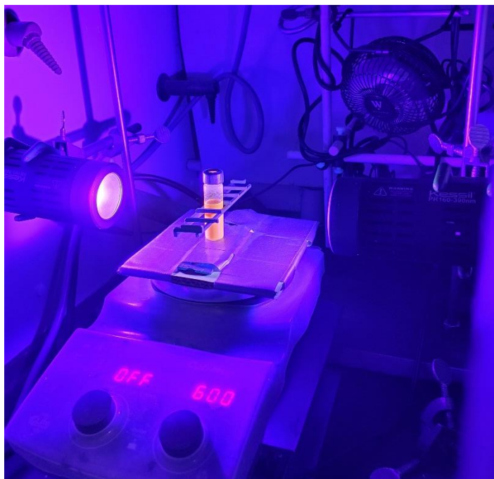
Figure S2: Photochemical Reaction Setup
