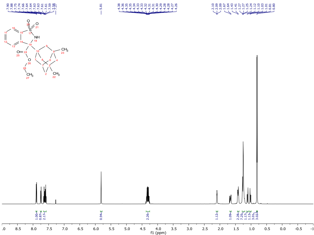
Compound 37 - 1H - 500MHz
