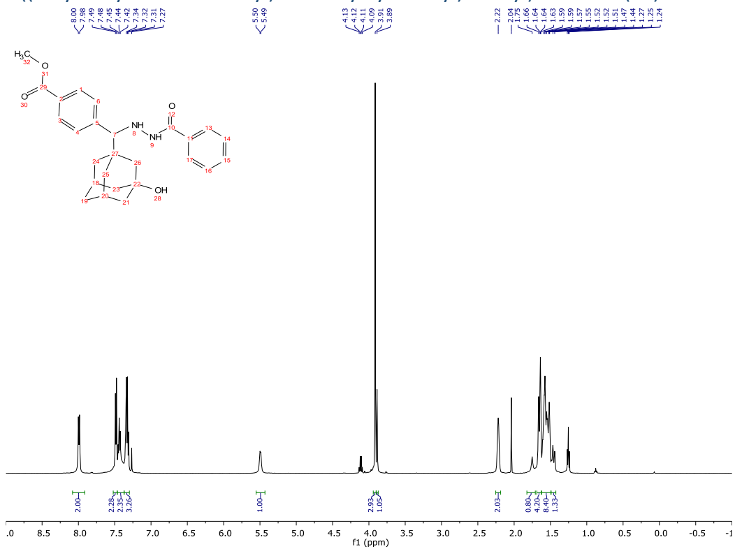
Compound 36 - 1H - 500MHz
