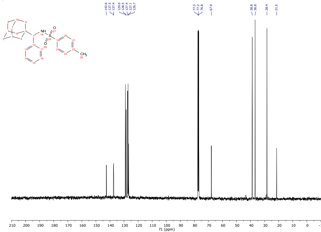
Compound 9 - 13C - 100MHz
