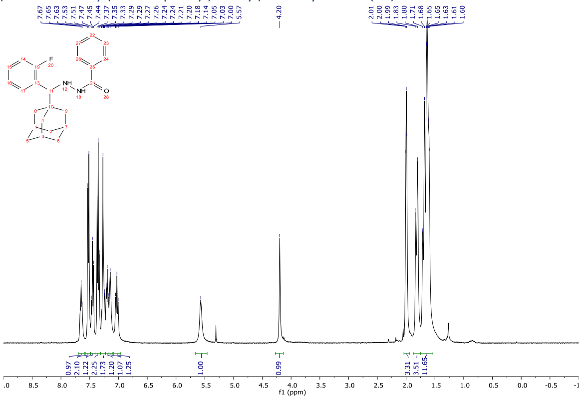
Compound 29 — 1H 400.13 MHz in CDCl 3
