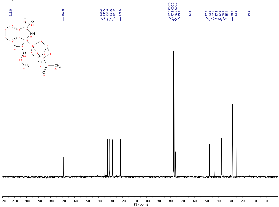
Compound 40 - 13C - 100MHz
