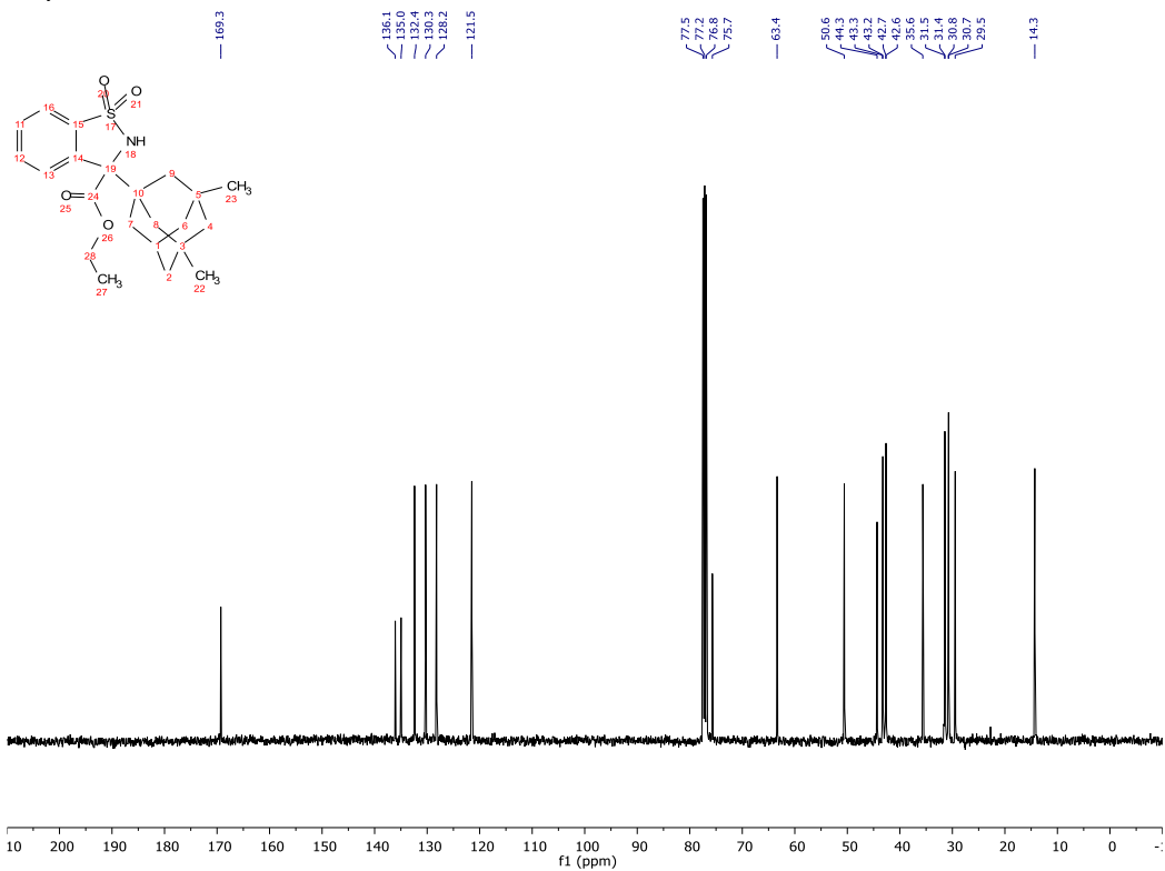
Compound 37 - 13C - 100MHz
