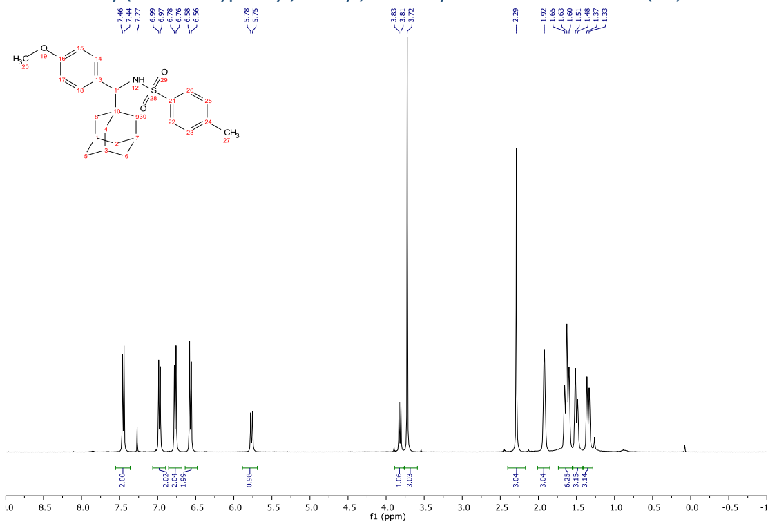
Compound 21 - 1H - 400 MHz
