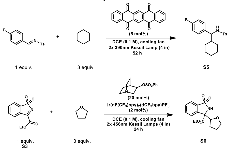
Scheme S2: Aminoalkylation of cyclohexane and tetrahydrofuran
