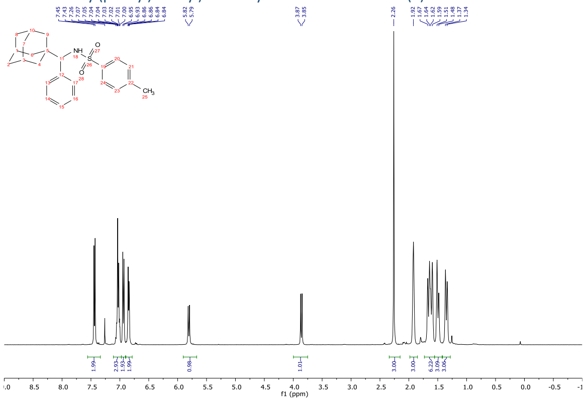
Compound 9 - 1H - 400MHz
