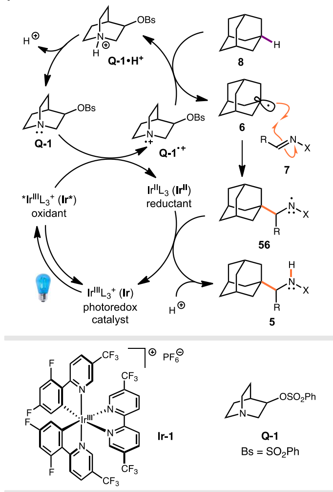
Scheme S1: Proposed Photocatalytic Cycle for Indirect HAT with Ir-1/Q-1
