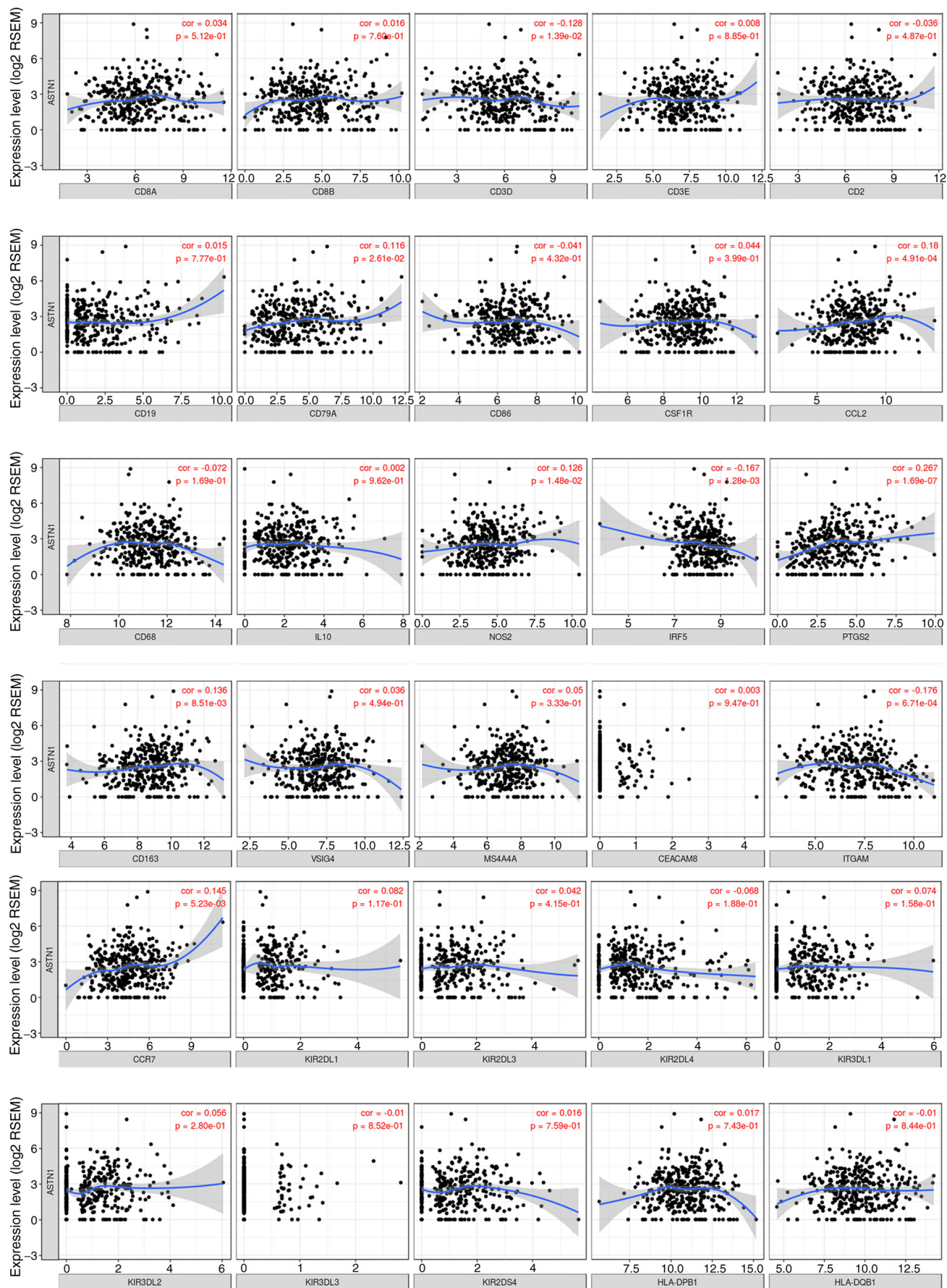
Figure S2. Correlation analysis between ASTN1 expression and immune marker genes. ASTN1, astrotactin 1.
