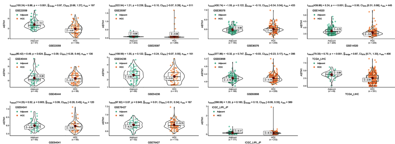
Figure S1. Differential expression of ASTN1 between HCC tissues and adjacent samples in HCCDB. ASTN1, astrotactin 1; HCC, hepatocellular carcinoma; HCCDB, Integrative Molecular Database of Hepatocellular Carcinoma.
