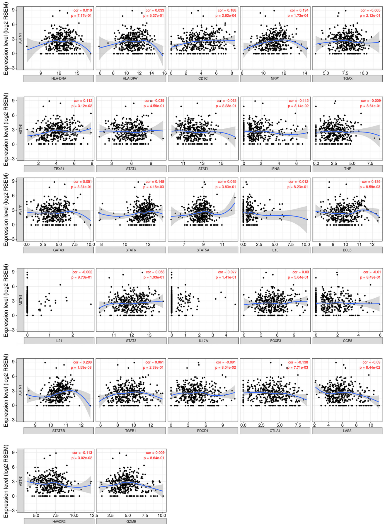
Figure S3. Correlation analysis between ASTN1 expression and immune marker genes. ASTN1, astrotactin 1.
