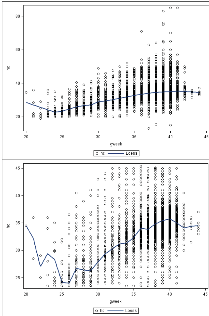
Appendix Figure 1. Head circumference by gestational week. Top, all data; bottom, implausible values removed.
