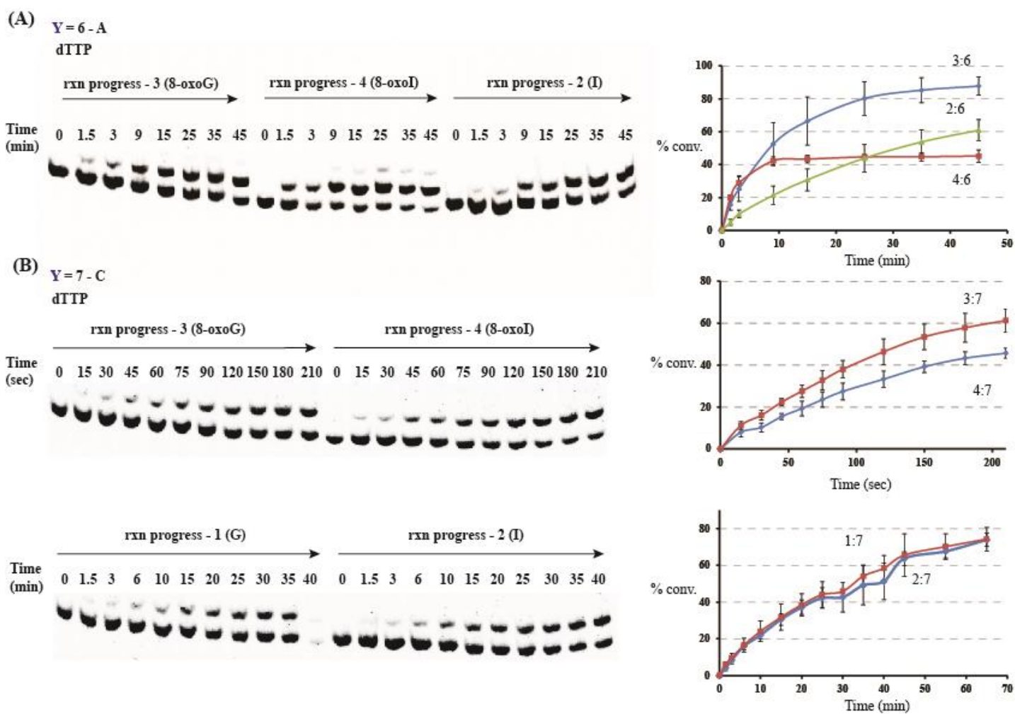
S 15 File. Relative rates for 2:6 – 4:6 with dTTP and 1:7 – 4:7 with dTTP at constant [dNTP] and [AMV-RT] as a function of time. Reactions carried out at rt.
