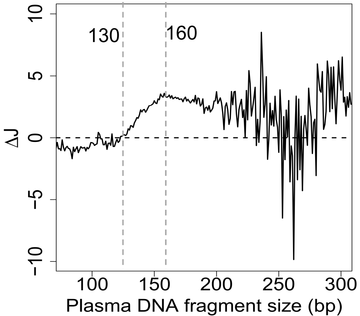
Fig. S5. The difference in JI-M ( \Delta J ) between the pooled shared (mainly of maternal origin) and fetal-specific DNA molecules against different sizes of plasma DNA. JI-M represents the jagged index deduced from methylated signals from CH sites.
