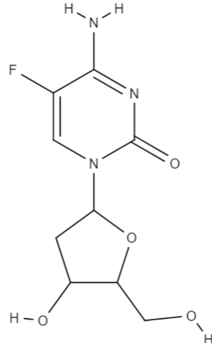
5'-fluoro-2'-deoxycytidine (FdCyd)
