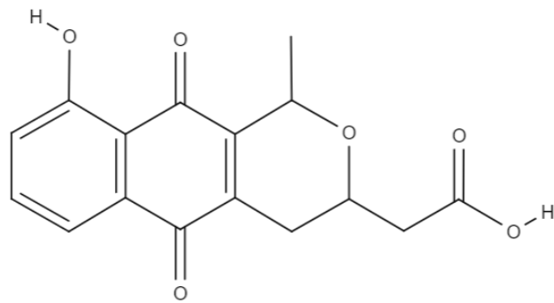
Nanaomycin A
