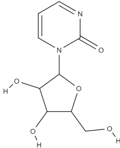
Zebularine
