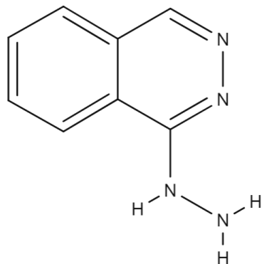
Hydralazine
