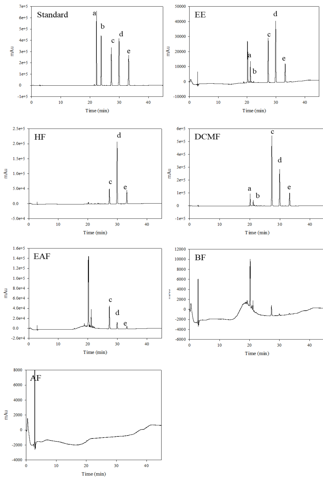
Figure S1. Chromatogram of Rumex crispus root extract and fractions at 420 nm. a: Aloe-emodin, b: Rhein, c: Emodin, d: Chrysophanol. e: Physcion (EE).
