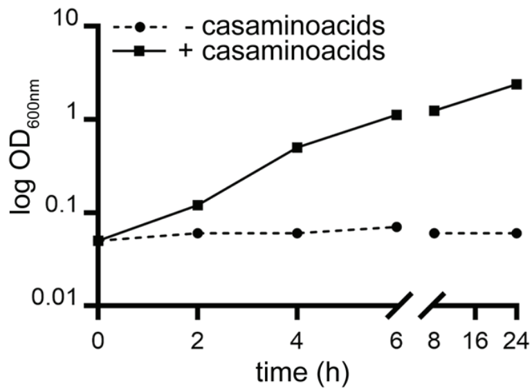
Supplementary Fig. S10. Growth of wild type S. Typhi after addition of casaminoacids. S. Typhi was grown for 24 hs in TTIM, and subsequently transferred to TTIM or to TTIM containing casaminoacids (1 %), which allows bacteria to re-enter the cell cycle. At the indicated time-points bacterial growth was monitored by measuring the OD 600 . This experiment was repeated at least three times with equivalent results.
