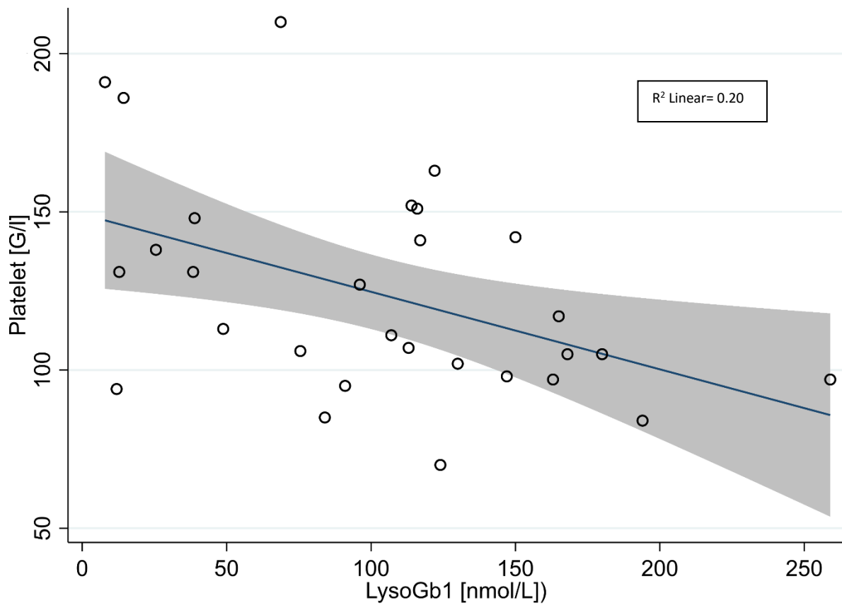
Figure S1. Correlation between lyso-Gb1 and platelet count at the last evaluation.
