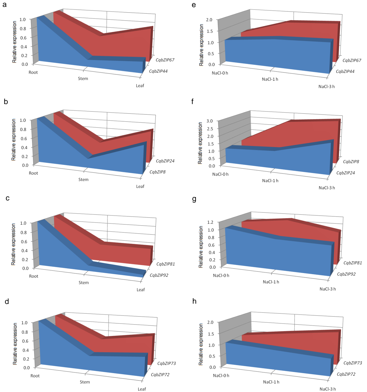
Additional file 10: Expression patterns of some duplicated CqbZIP genes in different organs ( a–d ) and in roots under salt stress treatment ( e–h ).
