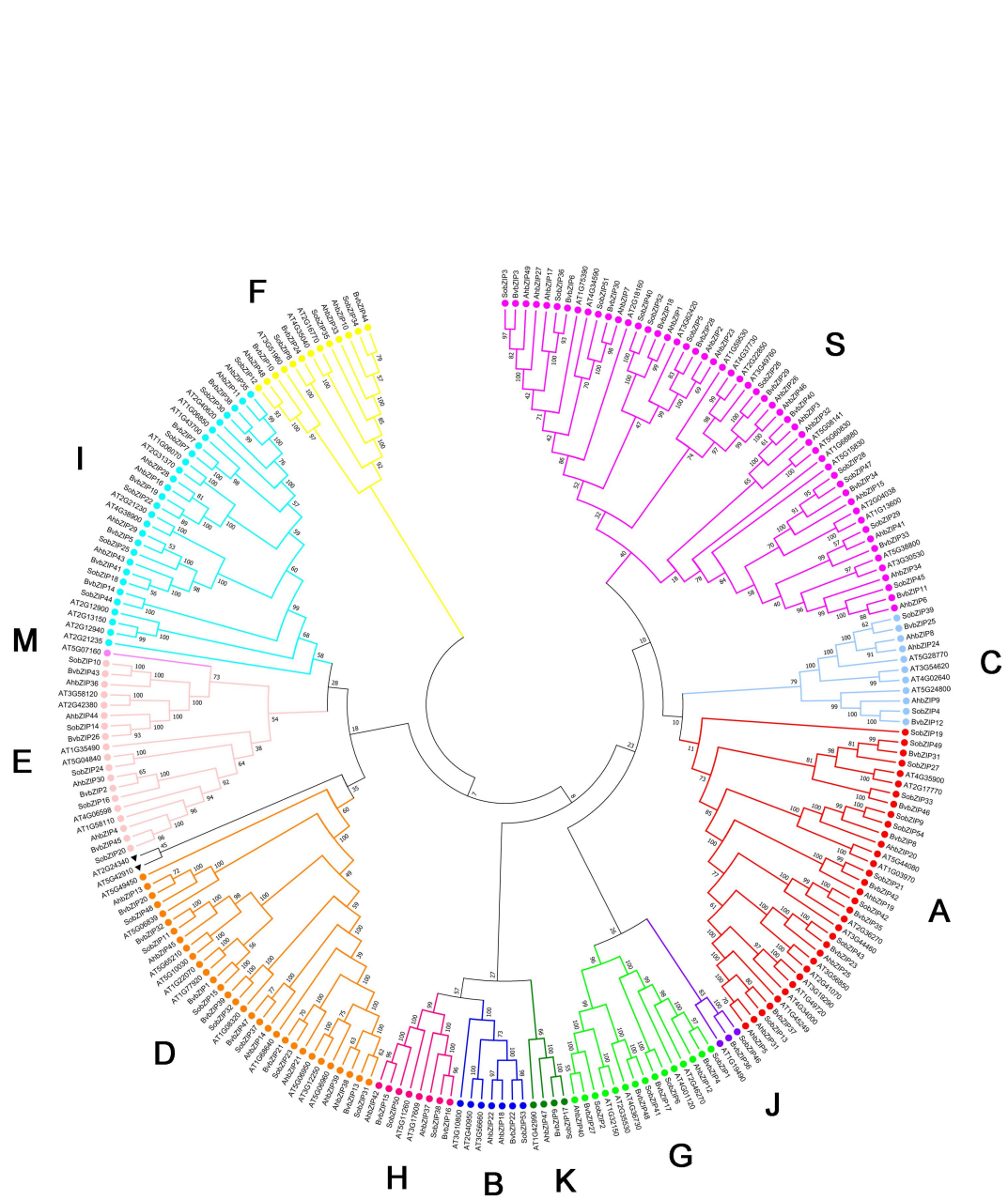
Additional file 5: Phylogenetic relationships of the bZIPs in spinach, beet, amaranth, and Arabidopsis.
