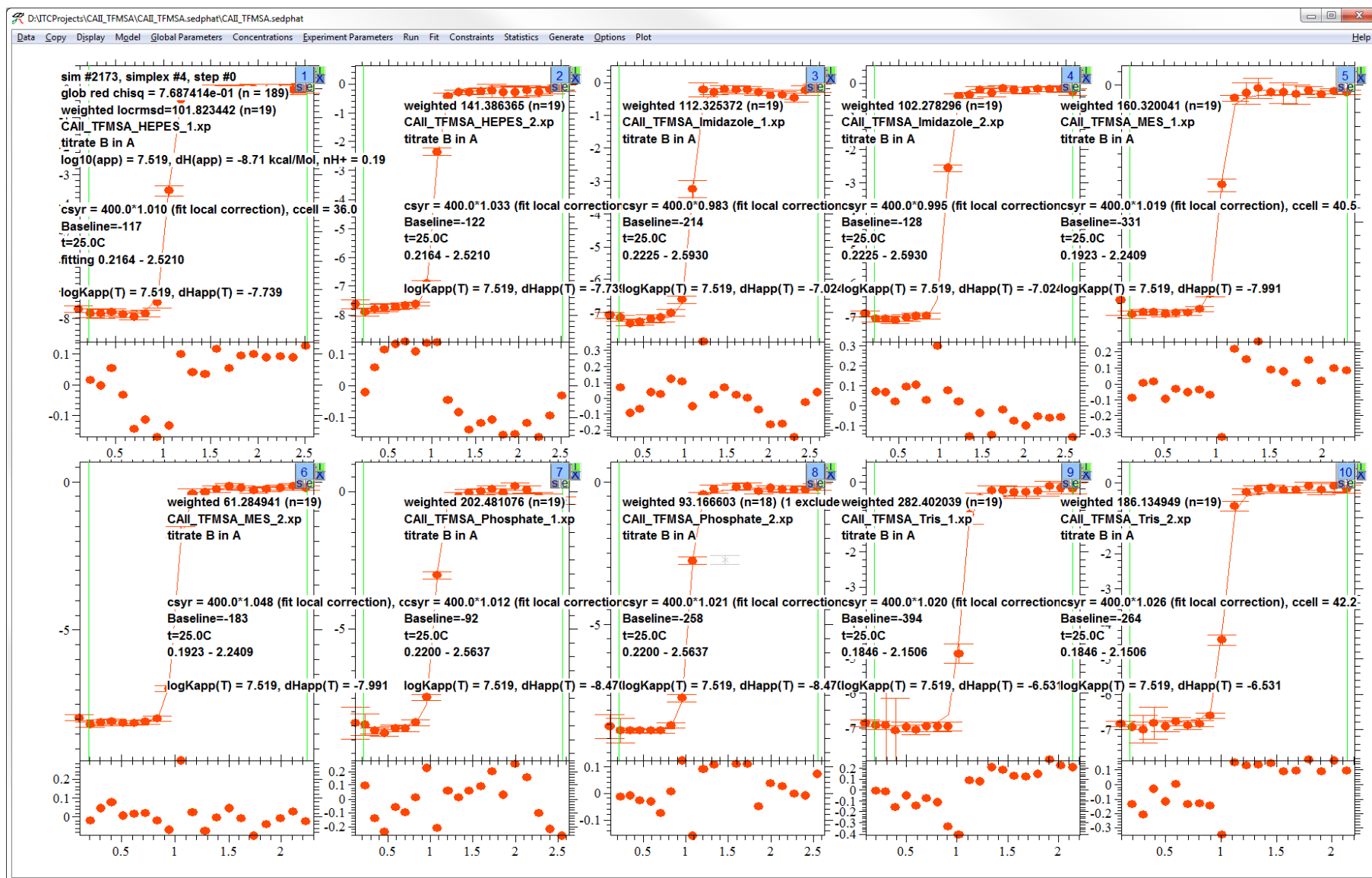
Supplementary Figure 1: Screenshot of the SEDPHAT window after fit has converged. In each experiment panel, the best-fit titration model is drawn as a solid line. For better inspection, the display can be freed of the textual output reporting global and local fit parameters by pressing ESC (it can be reproduced at any time by pressing control-O). It should be noted that the residuals are now on a reasonable scale, and for most experiments lack significant systematicity. The best-fit parameters can be obtained also in the model parameter box (control-P), or be summarized in a displayed ASCII text-file (control-T).
