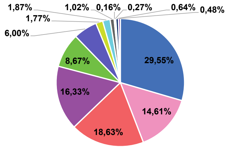
Supplementary Figure 1: Pie-chart of the chemical classes of compounds detected in potato periderms in positive (A) and negative (B) ionization modes as annotated by the ISDB-DNP and classified using ClassyFire.
