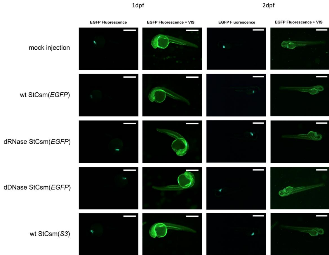
Figure S7: Tg(myI7:GFP) knockdown. Related to Figure 3. The effect of the injection of StCsm crRNA complexes into Tg(myI7:GFP) embryos was monitored.
