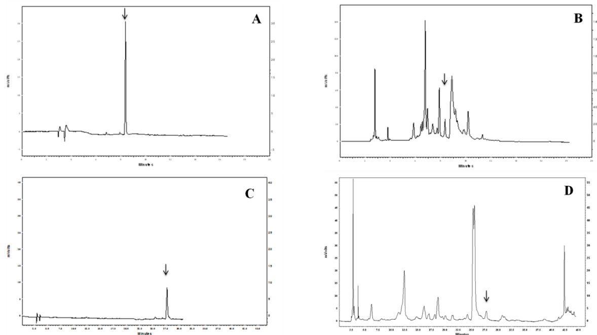
Figure S1. The high performance liquid chromatography (HPLC) chromatograms for measuring the contents of luteolin-7-O-glucoside and quercetin-7-O-glucoside in dandelion aqueous extract (DAE). (A) Standard luteolin-7-O-glucoside; (B) Luteolin-7-O-glucoside in DAE; (C) Standard quercetin-7-O-glucoside; (D) Quercetin-7-O-glucoside in DAE.
