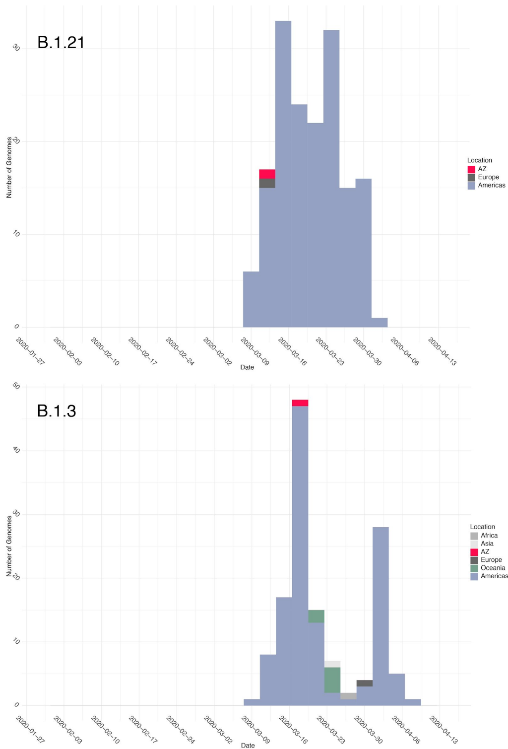
Figure S2. Sequence database representation through time for the 4 introductions with only 1 sequence representative from Arizona. Stacked bars are colored according to location. Lineages were assigned using Pangolin for all sequences uploaded to GISAID as of 4/16/2020.
