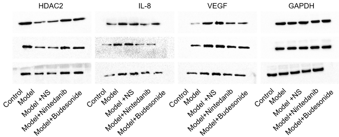
Supplementary Figure 1. Western blot analysis of HDAC2, IL-8 and VEGF proteins in tracheal tissues from rabbits after tracheal brushing and nintedanib treatments after using GAPDH as control. The blots were run independently three times and shown as three rows.
