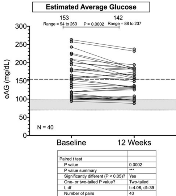
SUPPLEMENTARY FIG. S2. Individual subject glycemic values at baseline and completion of weeks 6 and 12.
