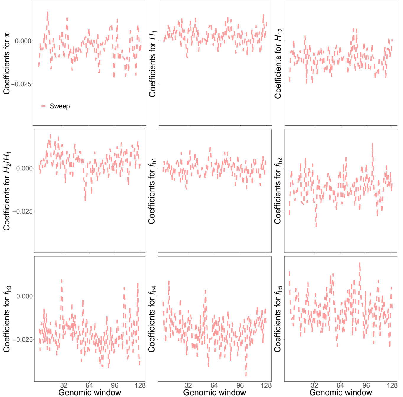
Figure S5: Reconstructed wavelets from regression coefficients ( \beta s) in sweep versus neutrality scenarios for summary statistics \hat{\pi} , H_1 , H_{12} , H_2/H_1 , and frequencies of first to fifth most common haplotypes for SURFDAWave when \gamma = 0 . SURFDAWave was trained on simulations of scenarios simulated under demographic specifications for European CEU demographic history. Note that the wavelet reconstructions for all summary statistics are plotted on the same scale, thereby making the distributions of some summaries difficult to decipher as their magnitudes are relatively small. SURFDAWave results shown are using Daubechies' least-asymmetric wavelets to estimate spatial distributions of summary statistics. Level 4 chosen through cross validation.
