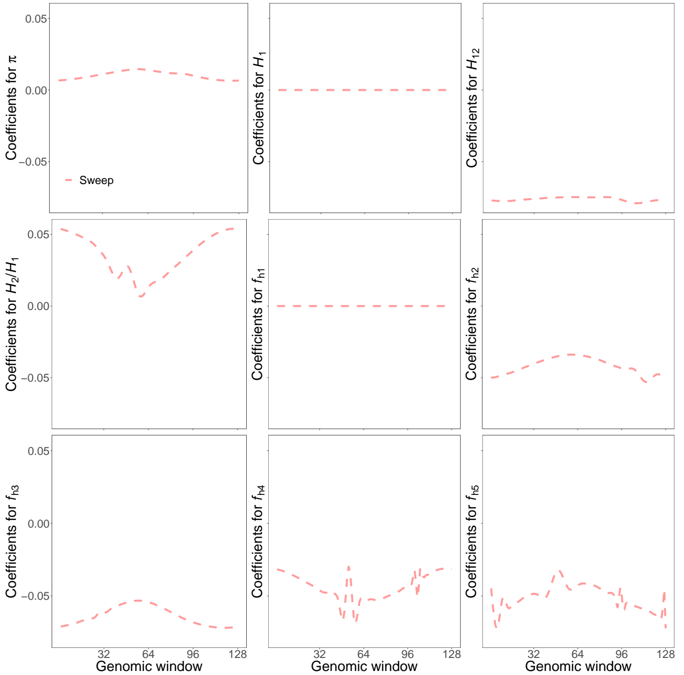
Figure S6: Reconstructed wavelets from regression coefficients ( \beta s) in sweep versus neutrality scenarios for summary statistics \hat{\pi} , H_1 , H_{12} , H_2/H_1 , and frequencies of first to fifth most common haplotypes for SURFDAWave when \gamma = 0.7 . SURFDAWave was trained on simulations of scenarios simulated under demographic specifications for European CEU demographic history. Note that the wavelet reconstructions for all summary statistics are plotted on the same scale, thereby making the distributions of some summaries difficult to decipher as their magnitudes are relatively small. SURFDAWave results shown are using Daubechies' least-asymmetric wavelets to estimate spatial distributions of summary statistics. Level 4 and \gamma = 0.7 chosen through cross validation.
