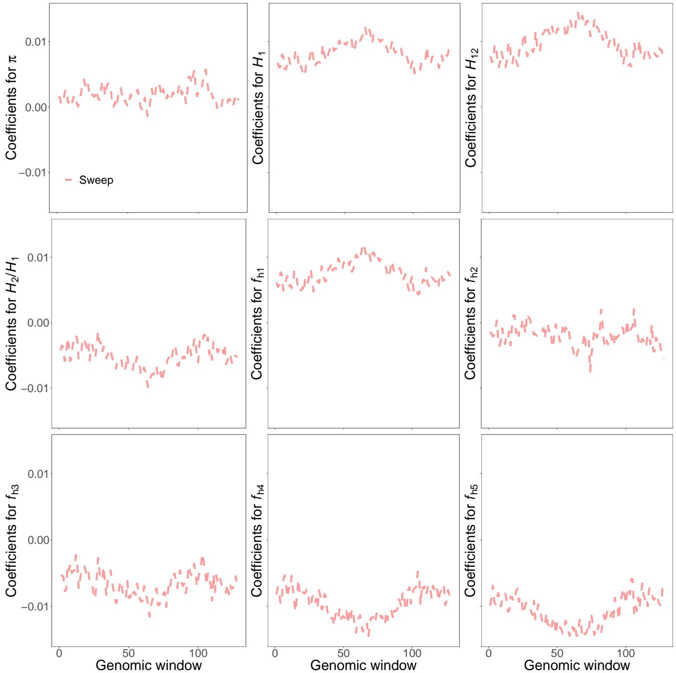
Figure S8: Reconstructed wavelets from regression coefficients ( \beta s) in sweep versus neutrality scenarios for summary statistics \hat{\pi} , H_1 , H_{12} , H_2/H_1 , and frequencies of first to fifth most common haplotypes for SURFDAWave when \gamma = 0 . SURFDAWave was trained on simulations of scenarios simulated under demographic specifications for sub-Saharan African YRI demographic history. Note that the wavelet reconstructions for all summary statistics are plotted on the same scale, thereby making the distributions of some summaries difficult to decipher as their magnitudes are relatively small. SURFDAWave results shown are using Daubechies' least-asymmetric wavelets to estimate spatial distributions of summary statistics. Level 4 chosen through cross validation.
