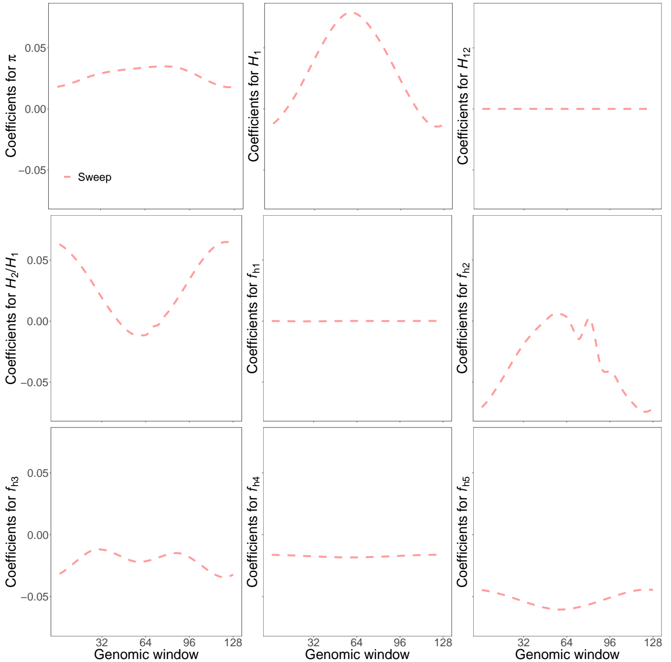
Figure S10: Reconstructed wavelets from regression coefficients ( \beta s) in sweep versus neutrality scenarios for summary statistics \hat{\pi} , H_1 , H_{12} , H_2/H_1 , and frequencies of first to fifth most common haplotypes for SURFDAWave when \gamma = 1 . SURFDAWave was trained on simulations of scenarios simulated under demographic specifications for sub-Saharan African YRI demographic history. Note that the wavelet reconstructions for all summary statistics are plotted on the same scale, thereby making the distributions of some summaries difficult to decipher as their magnitudes are relatively small. SURFDAWave results shown are using Daubechies' least-asymmetric wavelets to estimate spatial distributions of summmary statistics. Level 1 chosen through cross validation.
