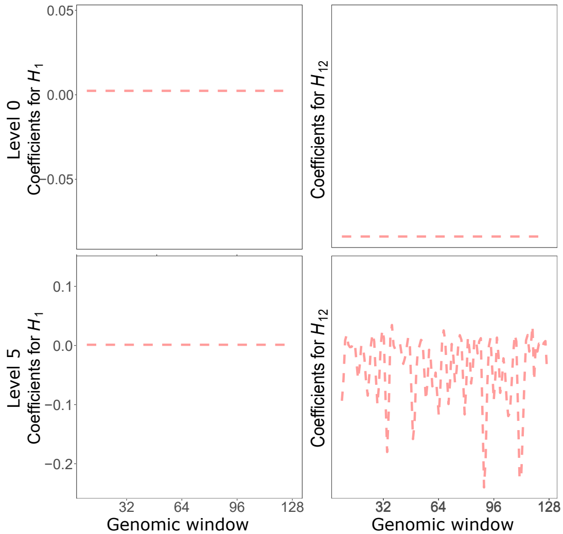
Figure S11: Reconstructed wavelets from regression coefficients ( \beta_s ) in sweep vs. neutrality scenarios for summary statistics H_1 and H_{12} showing difference between discrete wavelet transform at level 0 and level 5. Using Daubechies' least-Asymmetric wavelets and \gamma = 1 .
