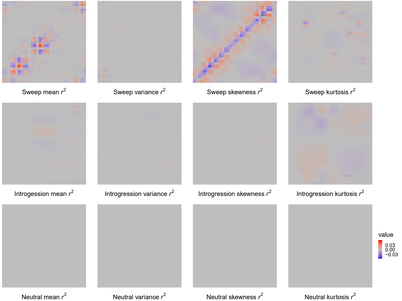
Figure S17: Reconstructed wavelets from regression coefficients ( \beta s) when differentiating among adaptive introgression, sweeps, and neutrality scenarios for summary statistics mean, variance, skewness, and kurtosis of pairwise r^2 for SURFDAWave when \gamma = 1 , when trained with statistics \hat{\pi} , H_1 , H_{12} , H_2/H_1 , and frequencies of first to fifth most common haplotypes (Figure S16). SURFDAWave was trained on simulations of scenarios simulated under demographic specifications for sub-Saharan African YRI demographic history. Note that the wavelet reconstructions for all summary statistics are plotted on the same scale, thereby making the distributions of some summaries difficult to decipher as their magnitudes are relatively small. SURFDAWave results shown are using Daubechies' least-asymmetric wavelets to estimate spatial distributions of summary statistics. Level 1 chosen through cross validation.
