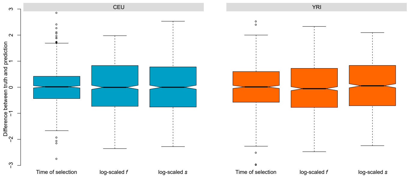
Figure S22: Difference between standardized predicted and actual selection parameters with SURFDAWave for the CEU and YRI demographic models. (Left box plot) Difference in prediction and truth of log scaled time at which mutation became beneficial. (Middle box plot) Difference in prediction and truth of log scaled frequency reached by mutation prior to it becoming beneficial ( f ). (Right box plot) Difference in prediction and truth of log scaled selection coefficient ( s ).
