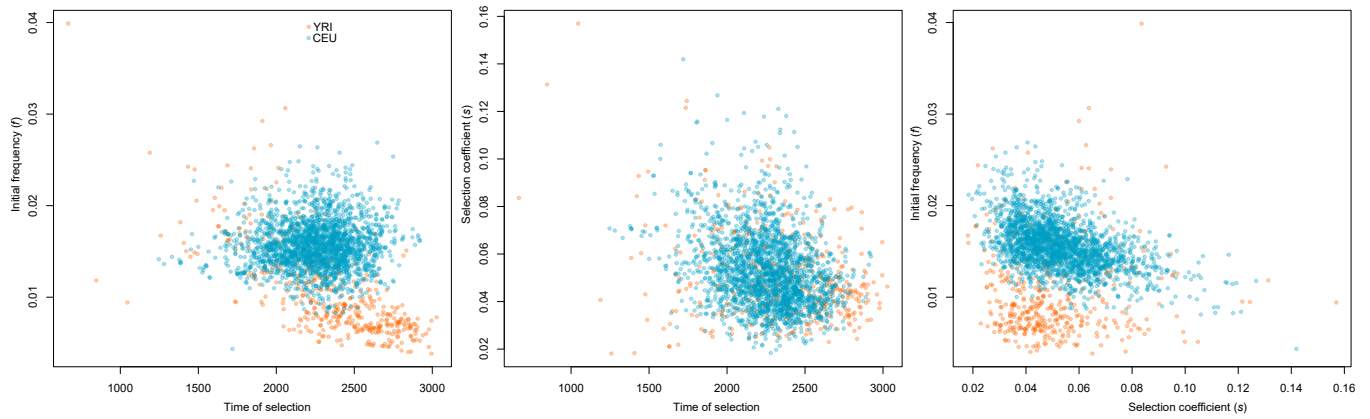
Figure S28: Predicted selection parameters for all genes in YRI and CEU with probability of being classified as sweep greater than 0.7 (Left) Scatter plot of predicted initial frequency mutation reached before becoming beneficial (Initial frequency) versus generations before present at which selection began (Time of selection). (Middle) Scatter plot of Selection coefficient versus Time of selection. (Right) Scatter plot of Initial frequency versus selection coefficient.
